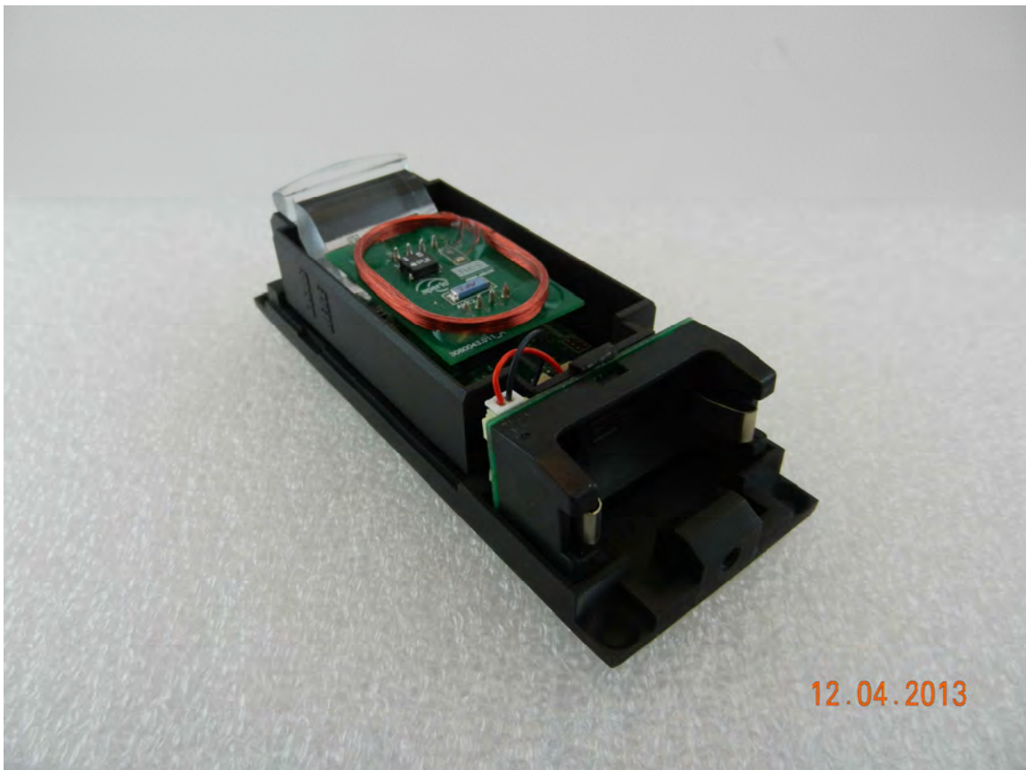
Assembled unit
