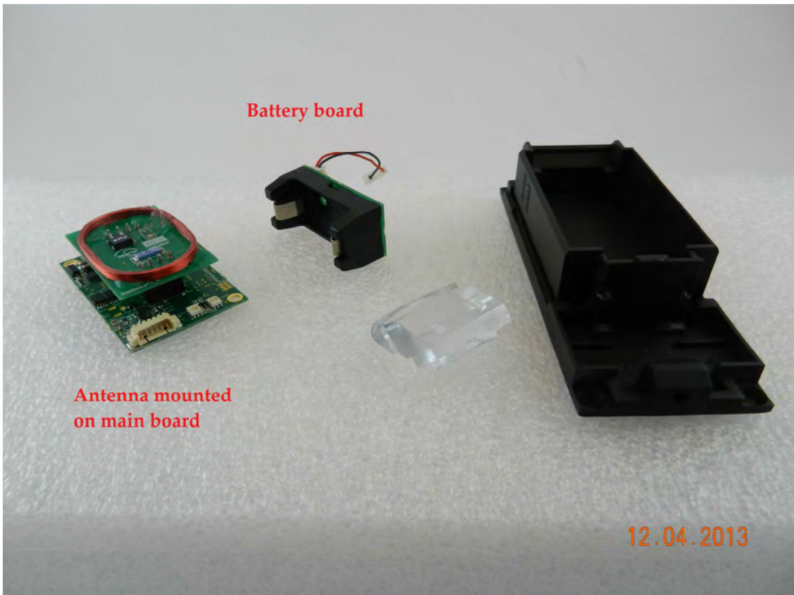
All boards with PCB tub and light guide
