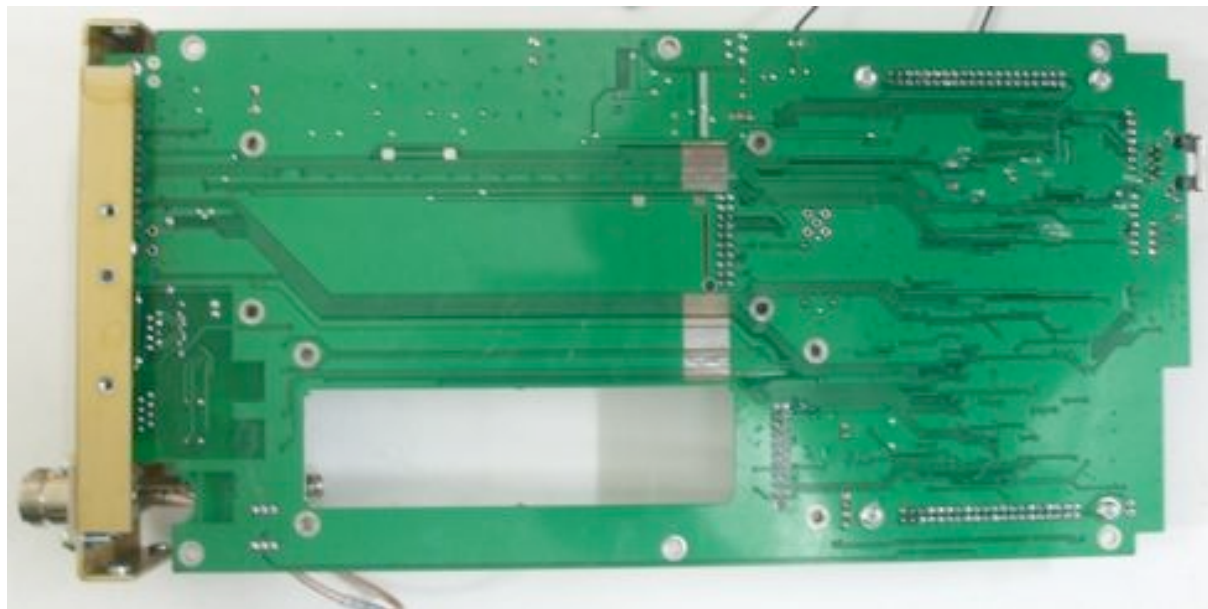
Main PCB
