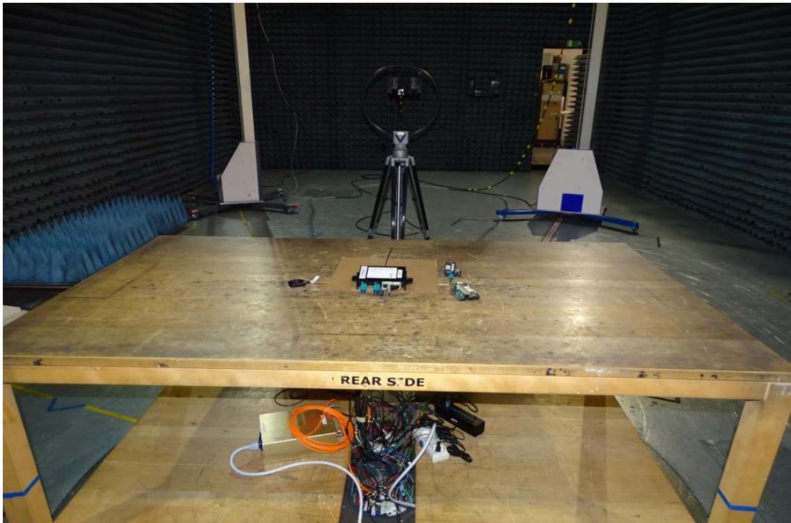
Photo 1: Test setup for radiated measurements below 30 MHz
