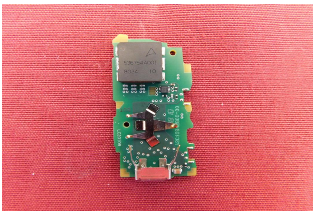
Picture 6: EUT module (top view)
