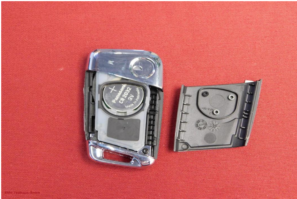
Picture 1: Opened FS14T, version FS14T with battery (top view)
