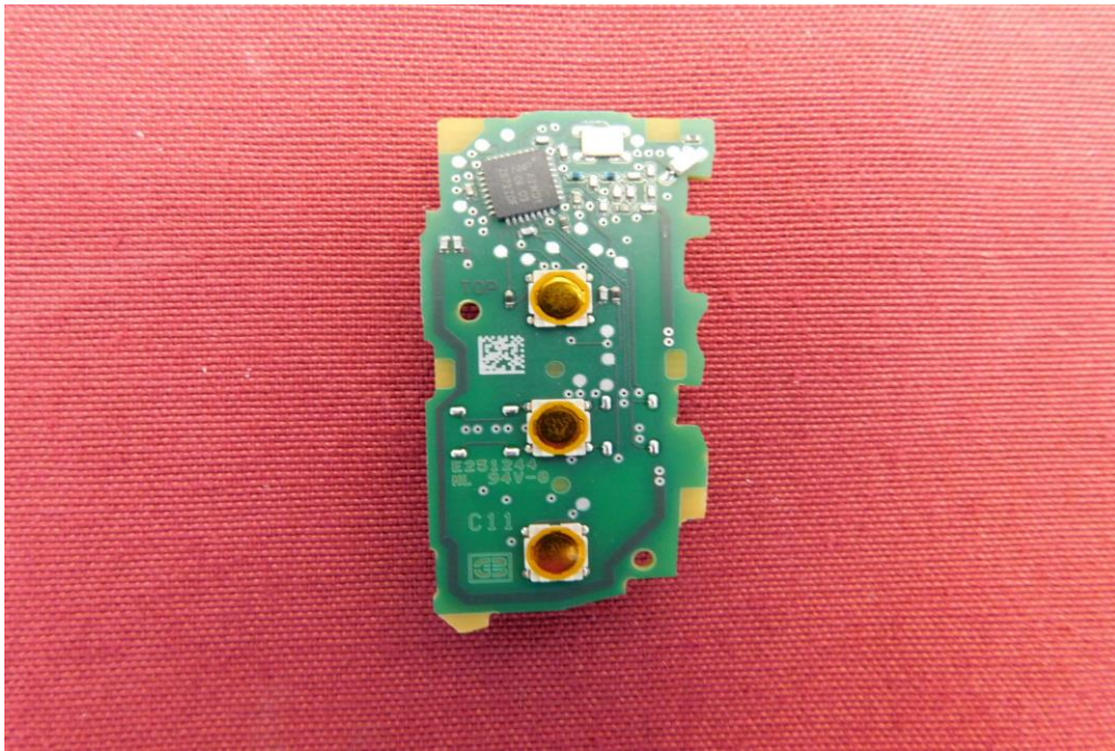
Picture 7: EUT module (back view)
