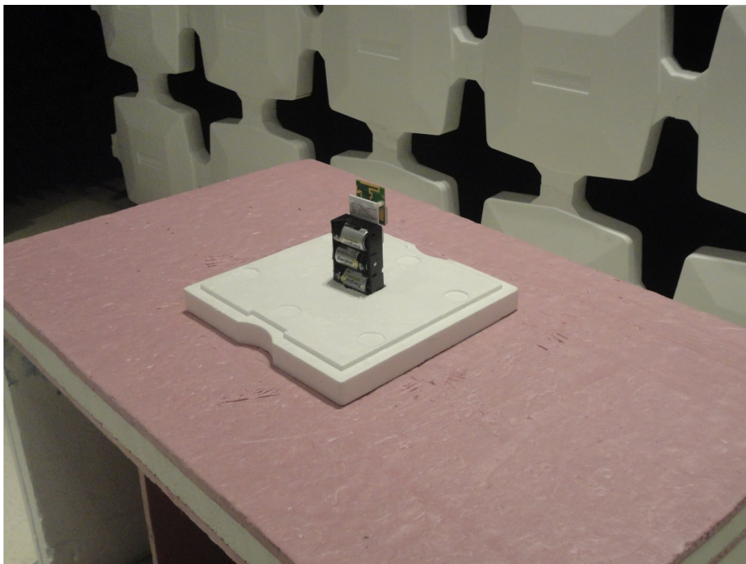
Radiated emissions integral antenna model
