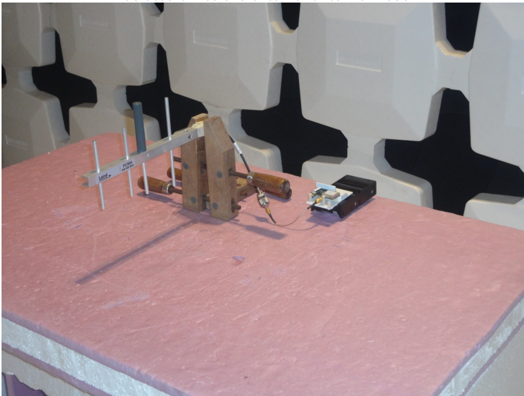
Radiated emissions external antenna model
