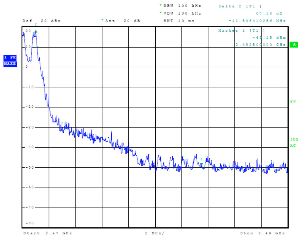
Figure Thirty-five Plot of High Band Edge (79 Hop Set)
