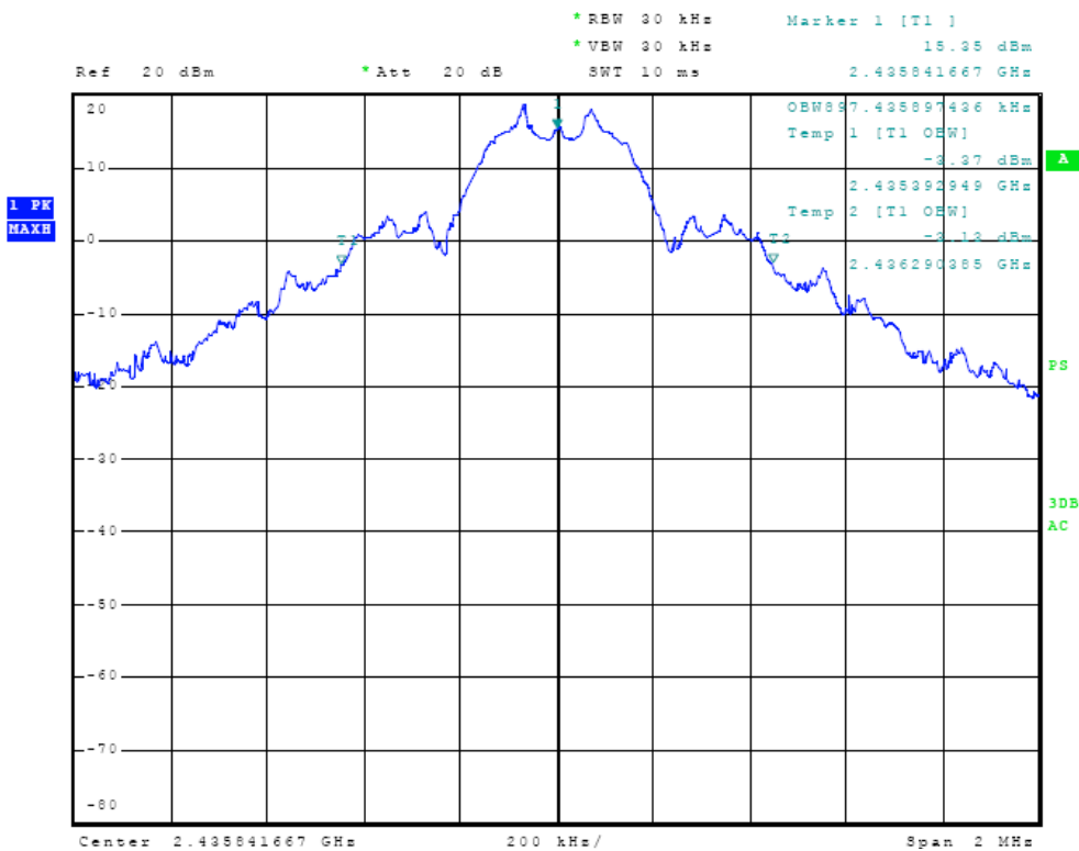
Figure Twenty-three Plot of 20 dB Occupied Bandwidth (79 Hop Set)
