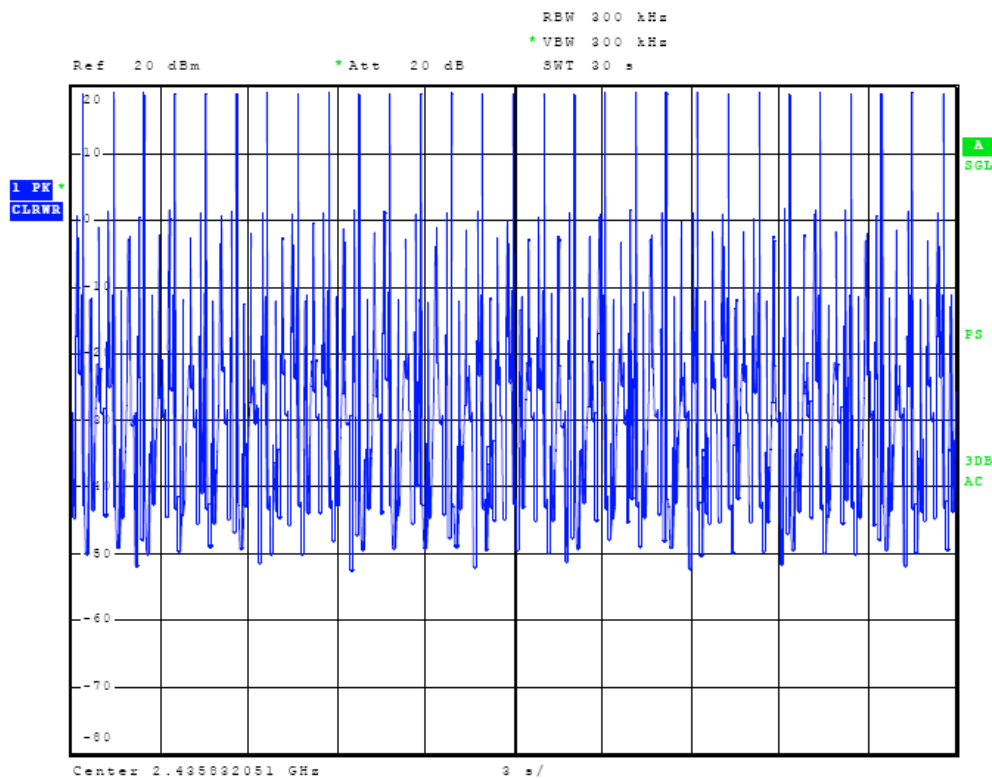
Figure Thirty-one Plot of Channel Occupancy (79 Hop Set)
