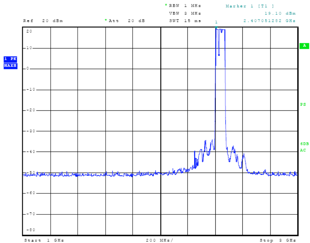
Figure Seventeen Plot of Antenna Port Conducted Emissions
