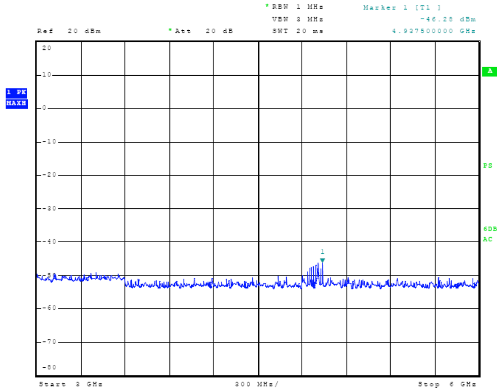
Figure Eighteen Plot of Antenna Port Conducted Emissions
