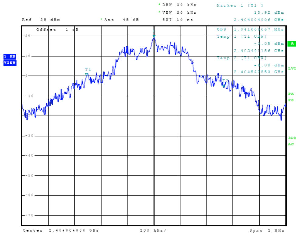
Figure Twenty-five Plot of 20 dB Occupied Bandwidth (43 Hop Set)
