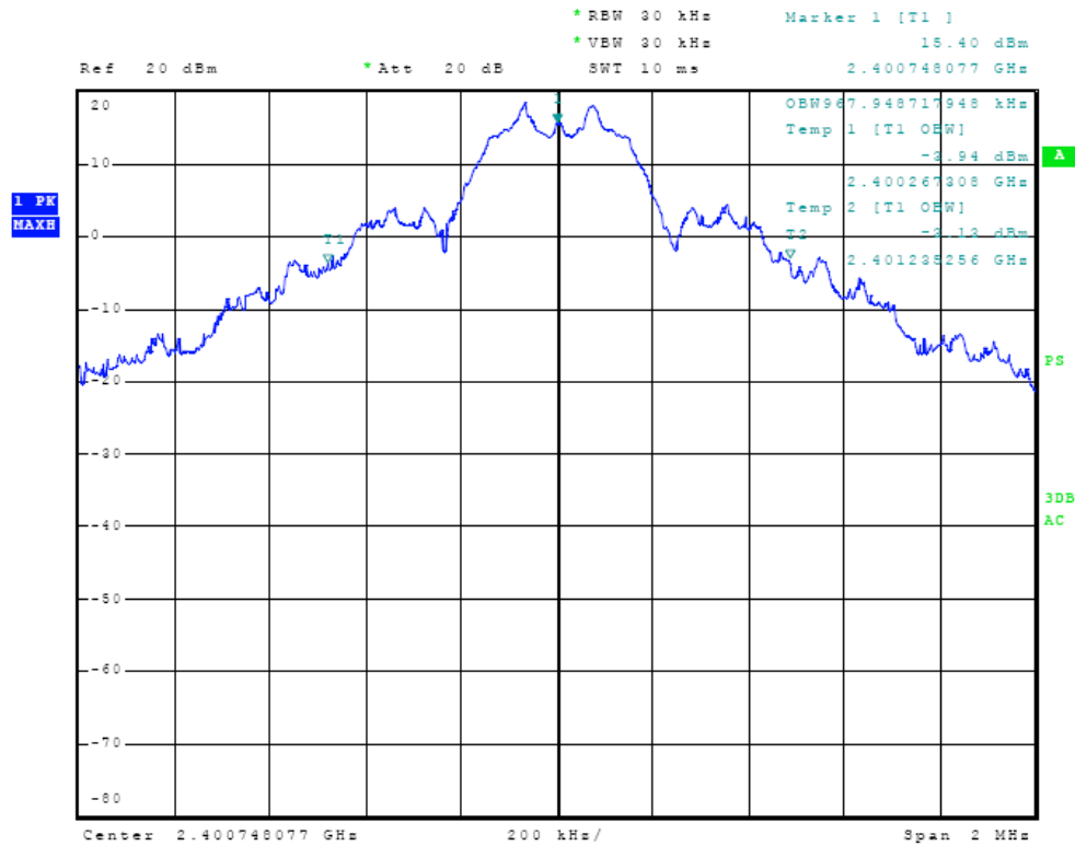
Figure Twenty-two Plot of 20 dB Occupied Bandwidth (79 Hop Set)
