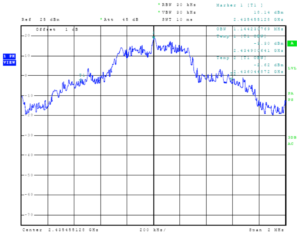
Figure Twenty-six Plot of 20 dB Occupied Bandwidth (43 Hop Set)
