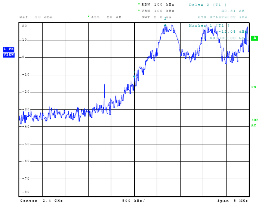
Figure Thirty-four Plot of Low Band Edge (79 Hop Set)
