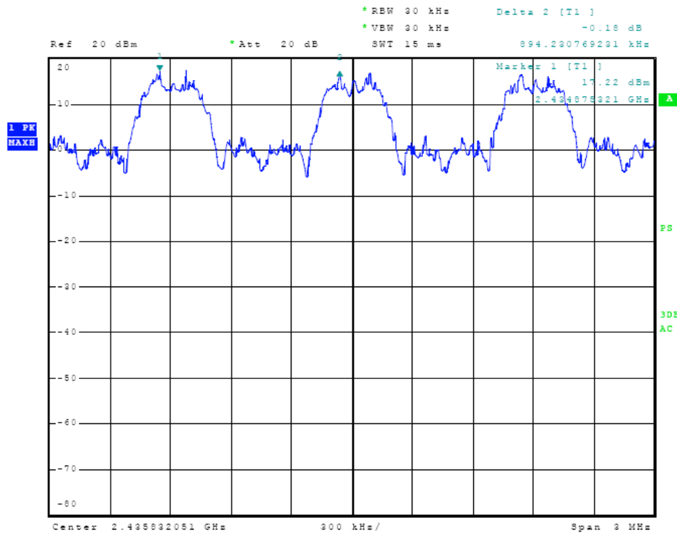
Figure Twenty-eight Plot of Channel Spacing (79 Hop Set)
