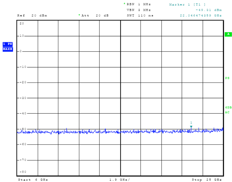
Figure Nineteen Plot of Antenna Port Conducted Emissions
