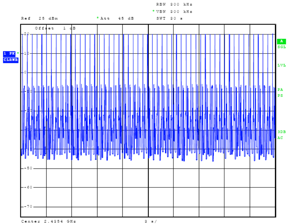
Figure Thirty-three Plot of Channel Occupancy (43 Hop Set)
