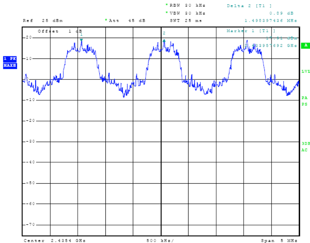
Figure Twenty-nine Plot of Channel Spacing (43 Hop Set)
