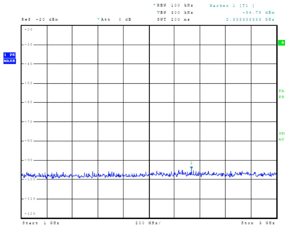
Figure Eleven Receiver Temporary Antenna Port Conducted Emissions
