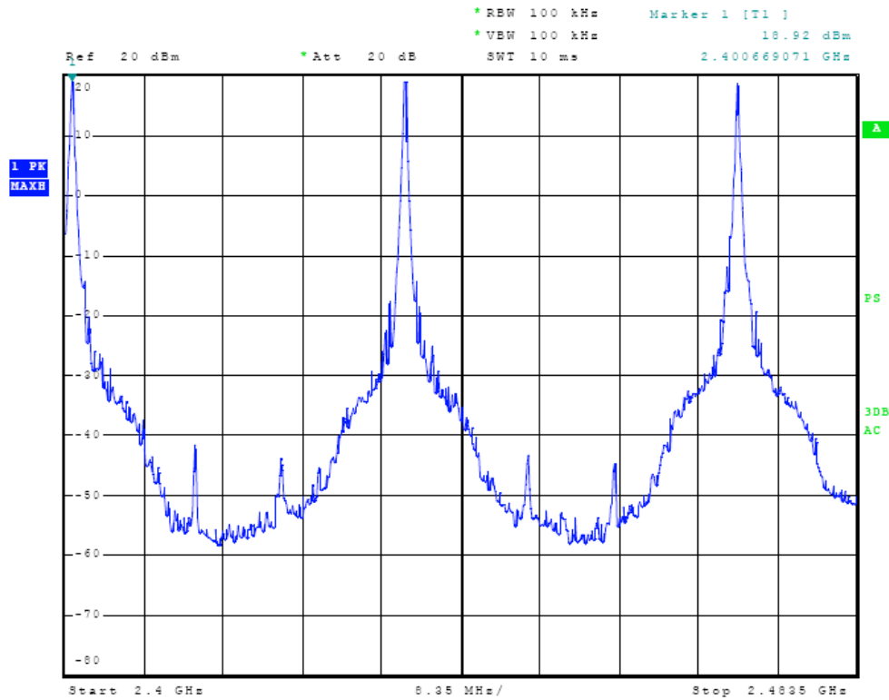
Figure Twenty Plot of Operation Across Operational Band (79 Hop Set)
