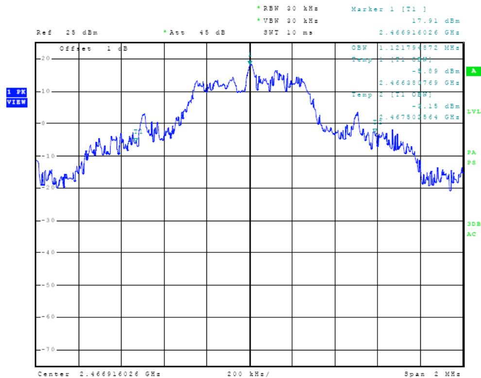
Figure Twenty-seven Plot of 20 dB Occupied Bandwidth (43 Hop Set)
