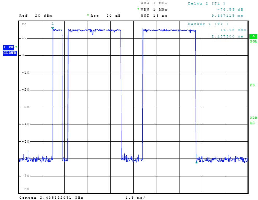
Figure Thirty Plot of Dwell time on Channel (79 Hop Set)
