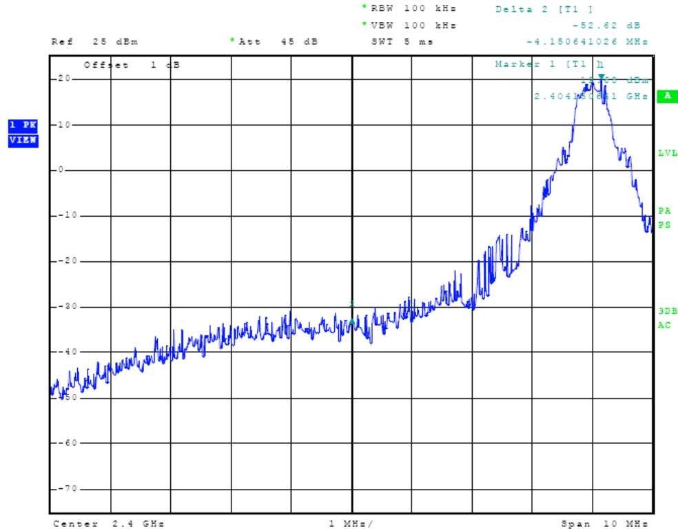
Figure Thirty-six Plot of Low Band Edge (43 Hop Set)
