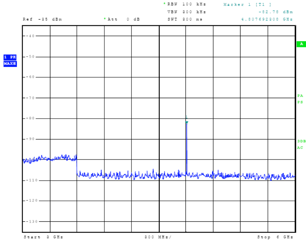
Figure Twelve Receiver Antenna Port Conducted Emissions
