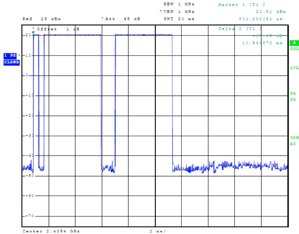
Figure Thirty-two Plot of Plot of Dwell time on Channel (43 Hop Set)
