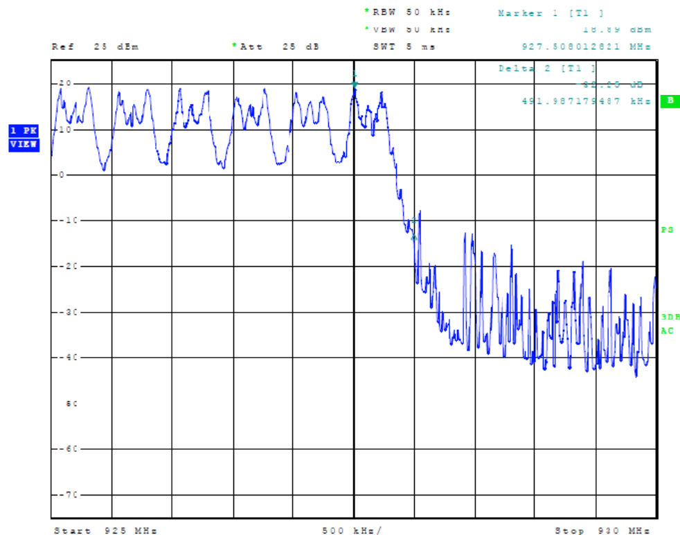
Figure Twenty Plot of High Band Edge
