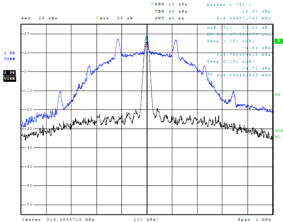
Figure Fourteen Plot of 20-dB Occupied Bandwidth (Middle Channel)
