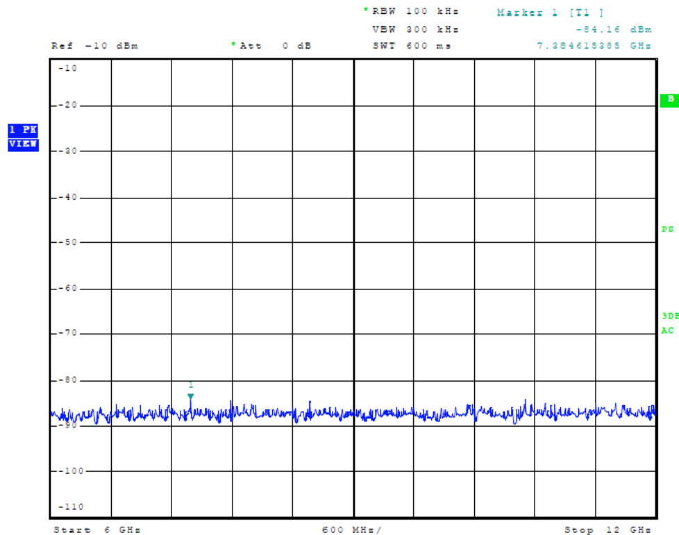
Figure Twenty-four Receiver Antenna Port Conducted Emissions
