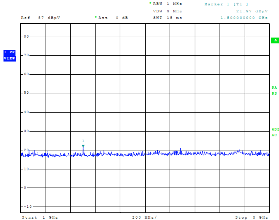
Figure Twenty-seven Plot of Receiver Radiated Spurious Emissions taken at 1 meter
