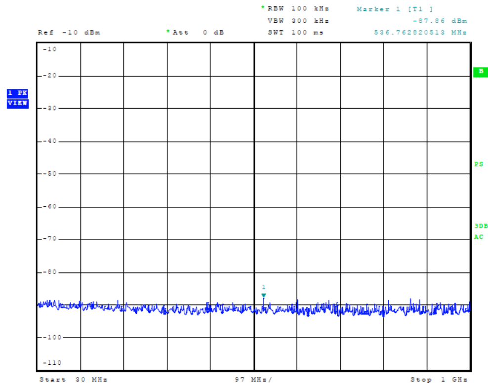
Figure Twenty-one Receiver Antenna Port Conducted Emissions
