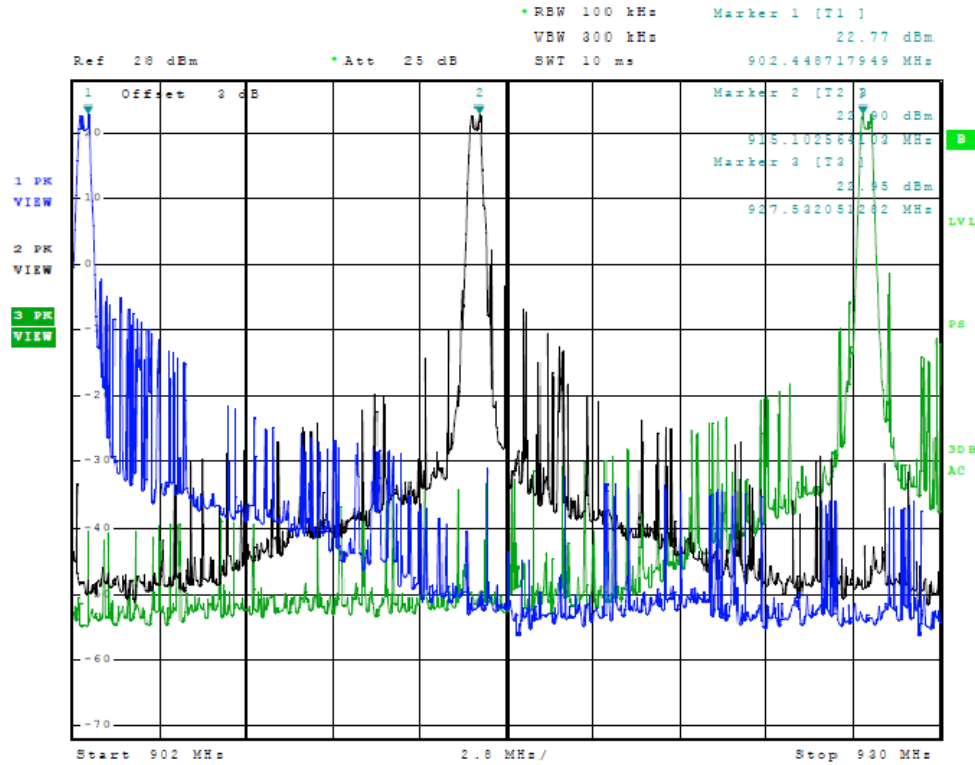
Figure Twelve Plot of Output Across Operational Band
