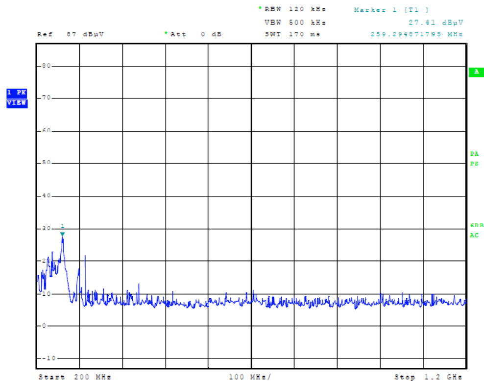
Figure Twenty-six Plot of Receiver Radiated Spurious Emissions taken at 1 meter
