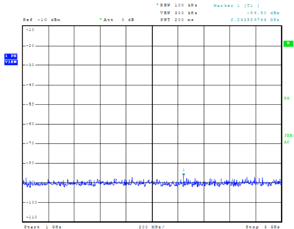
Figure Twenty-two Receiver Antenna Port Conducted Emissions
