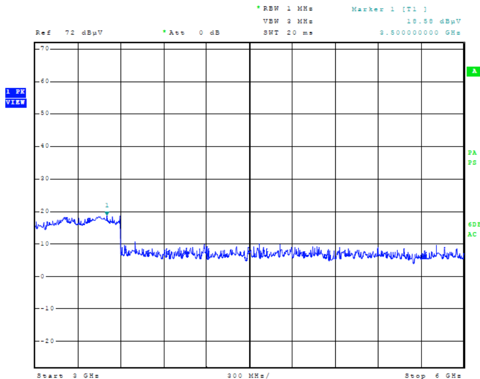
Figure Twenty-eight Plot of Receiver Radiated Spurious Emissions taken at 1 meter
