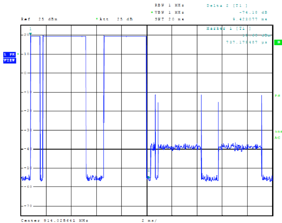
Figure Seventeen Plot of Dwell time on Channel
