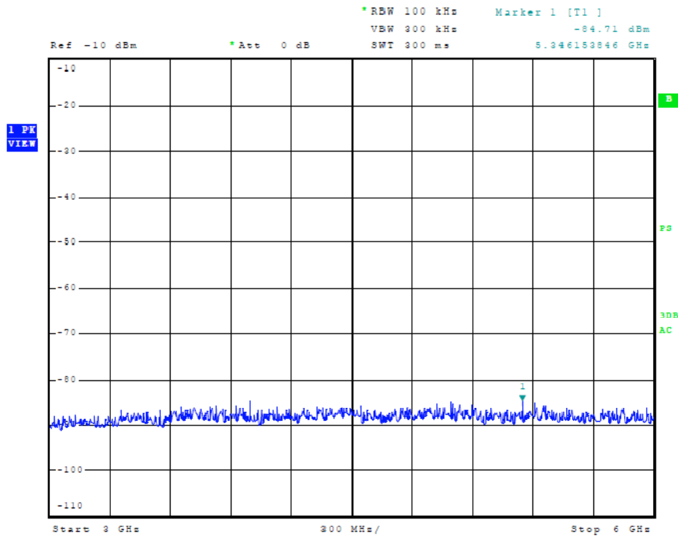
Figure Twenty-three Receiver Antenna Port Conducted Emissions
