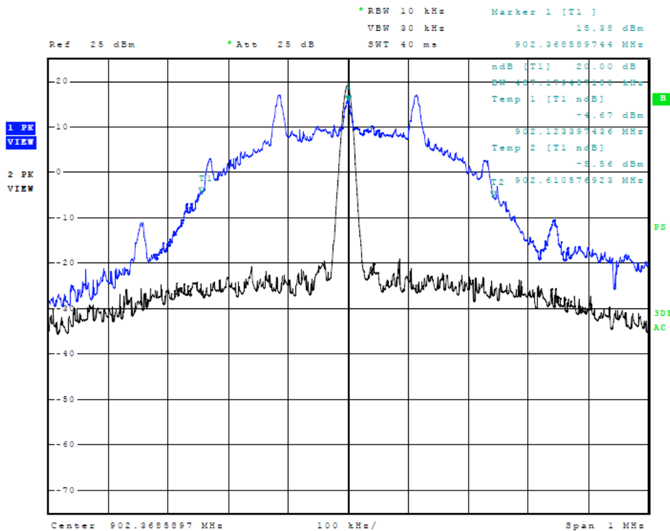
Figure Thirteen Plot of 20-dB Occupied Bandwidth (Low Channel)
