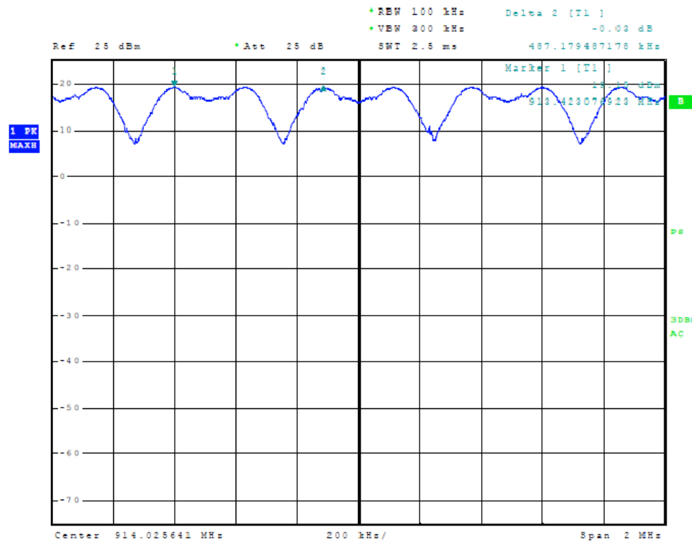
Figure Sixteen Plot Channel Spacing
