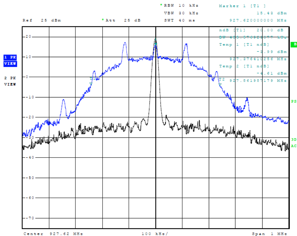
Figure Fifteen Plot of 20-dB Occupied Bandwidth (High Channel)
