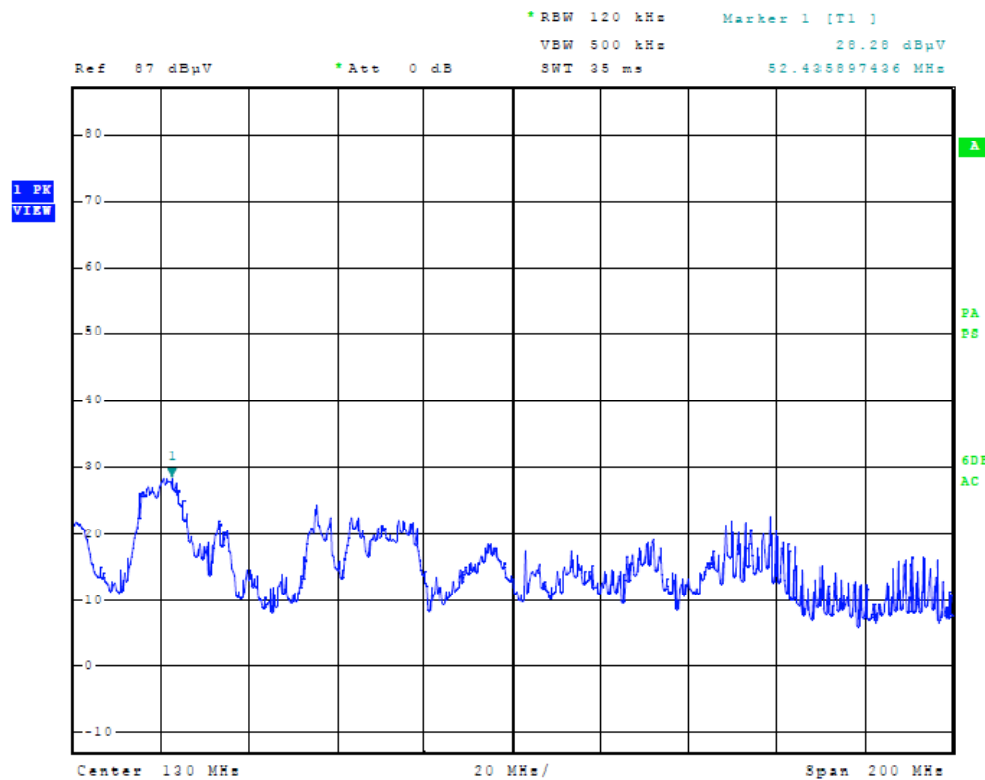
Figure Twenty-five Plot of Receiver Radiated Spurious Emissions taken at 1 meter
