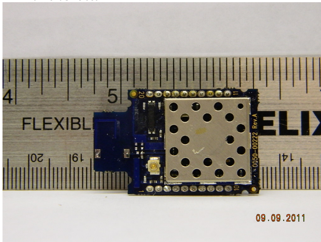
PRM240 Front Shielded
