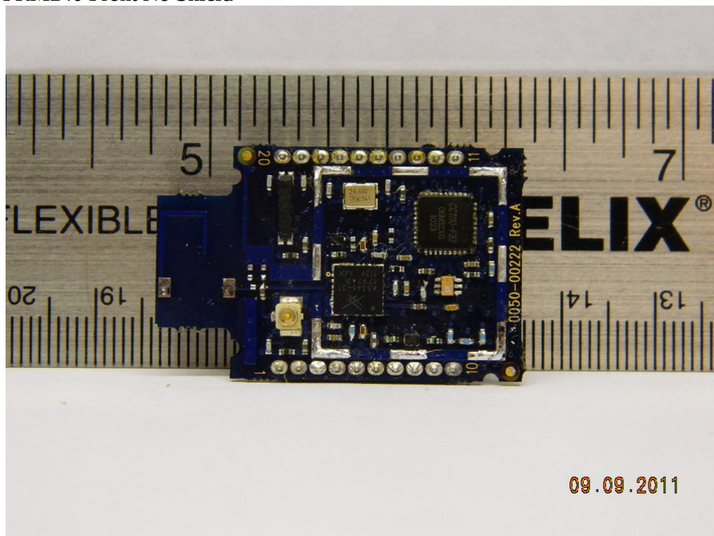
PRM240 Front No Shield
