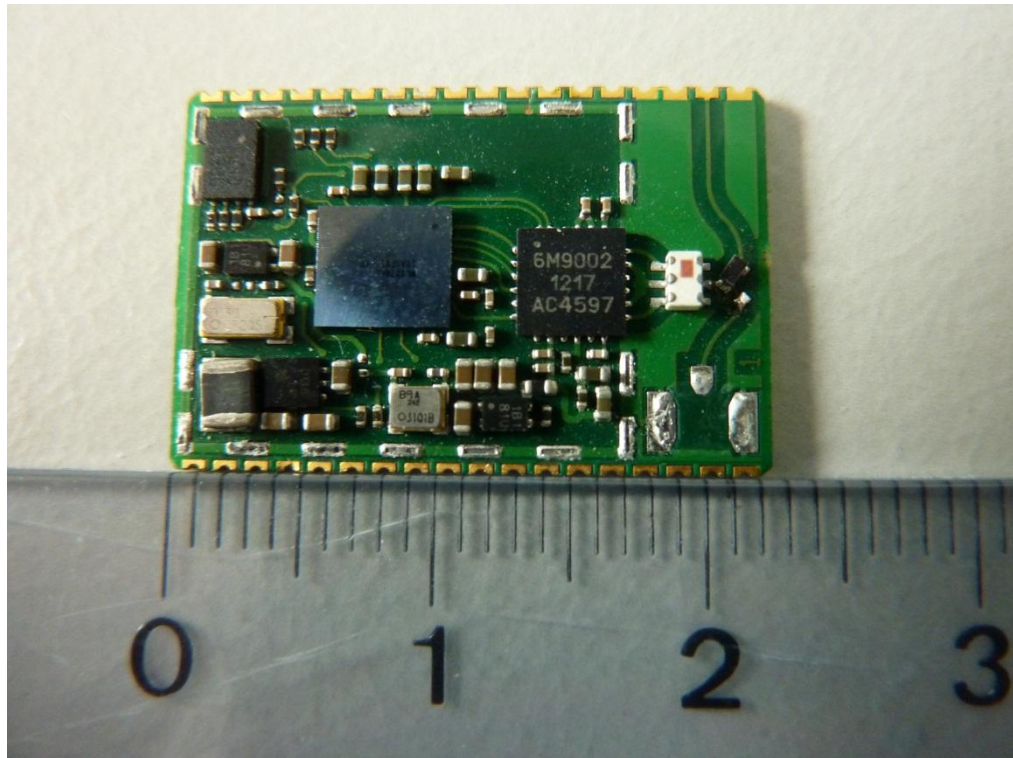
145298_25.JPG: EUT - top view, shielding removed
