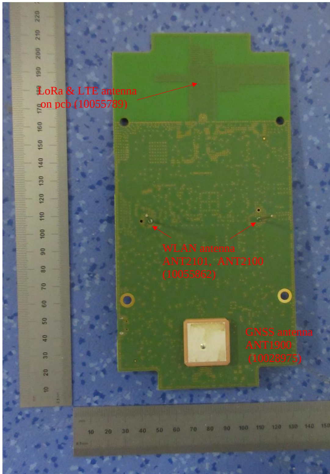
FULL SLBB board (10050364)
