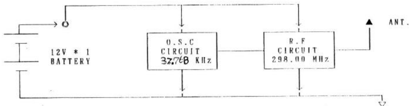
PERSONAL PAGER TRANSMITTER BLOCK DIAGRAM
