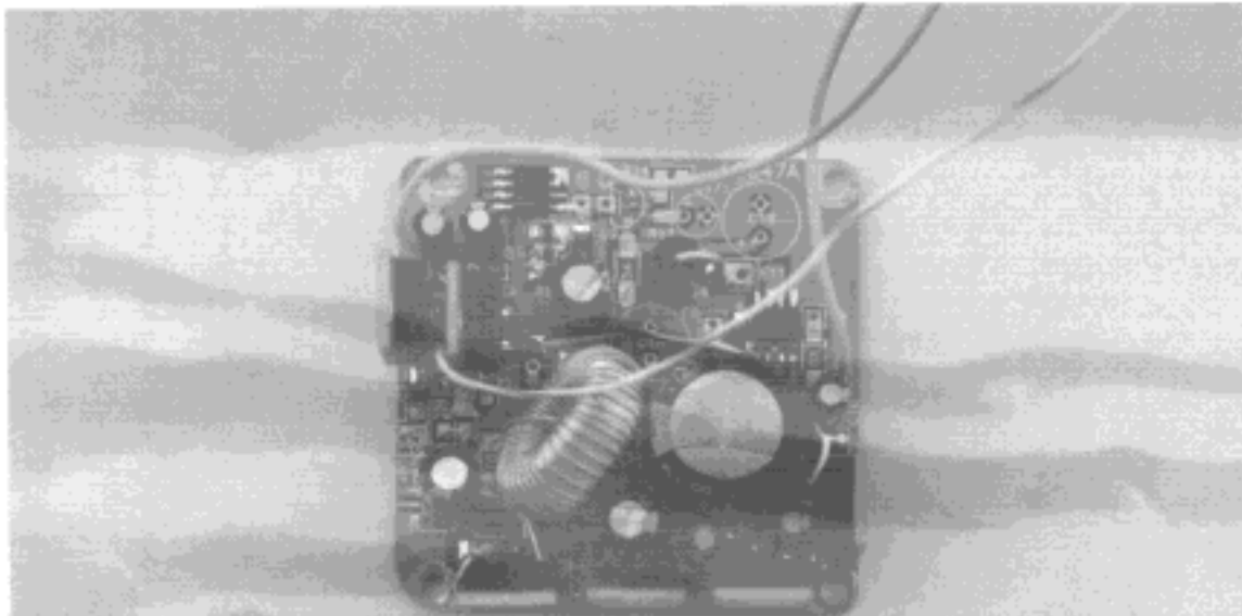
S-Band Power Supply Board - Top
