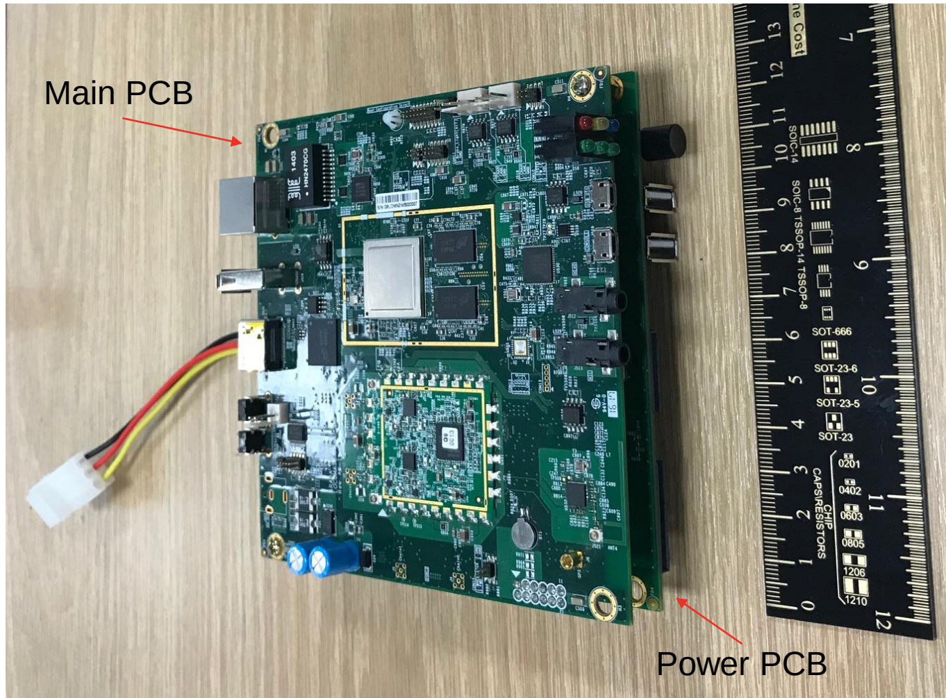
PCB Assembly (Main PCB + Power PCB)
