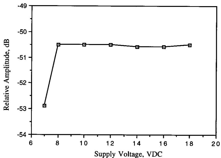
Figure 6.2. Relative emission at "fundamental" vs. supply voltage.
