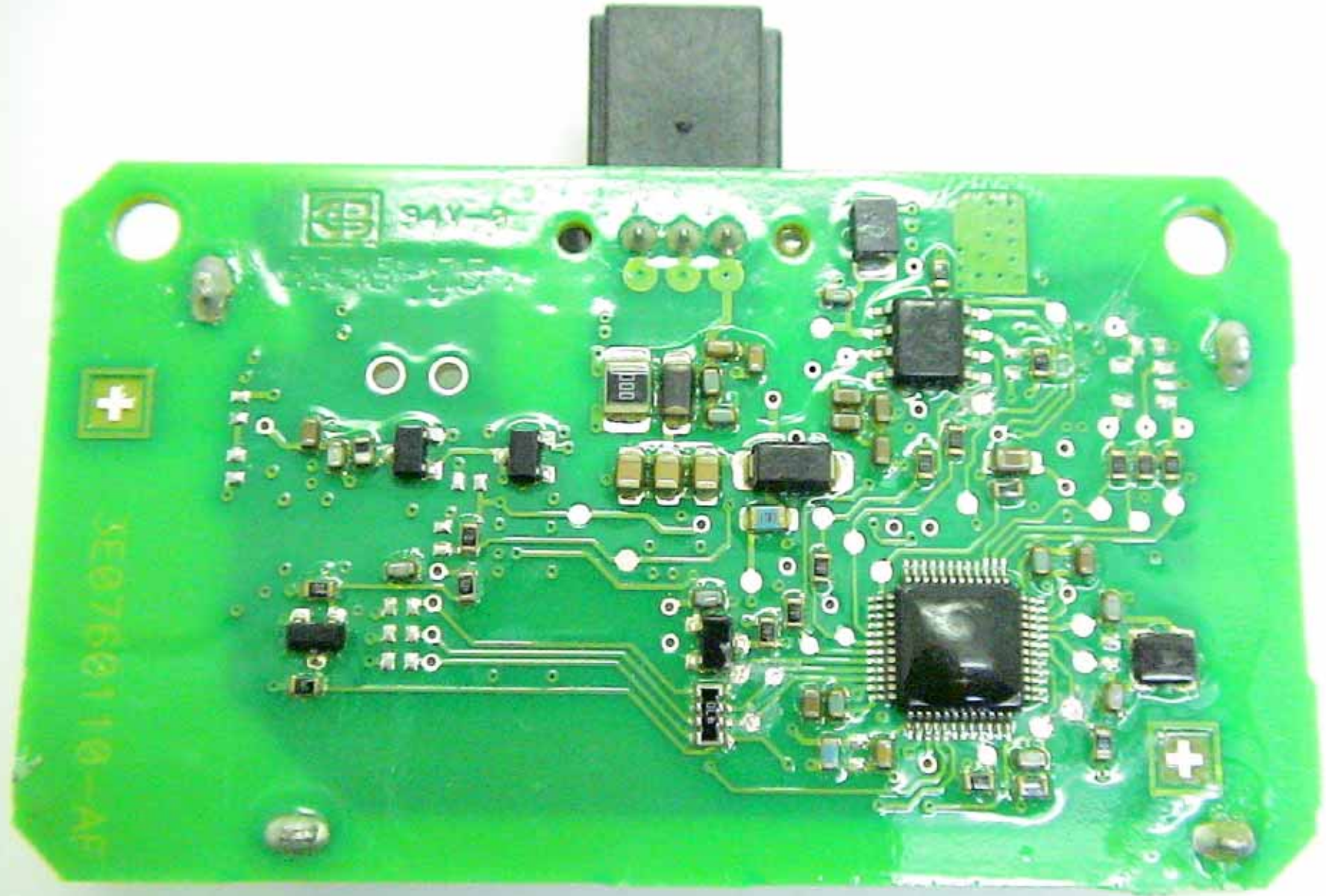
PCB (bottom)
