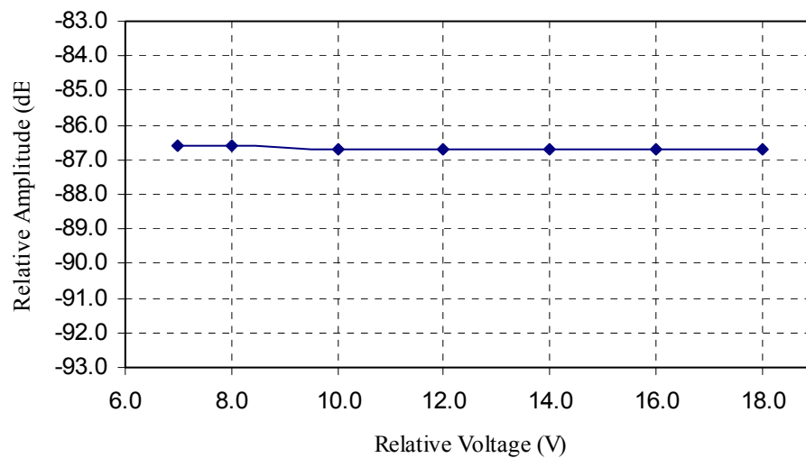
Figure 6.2. Relative emission at "fundamental" vs. supply voltage.
