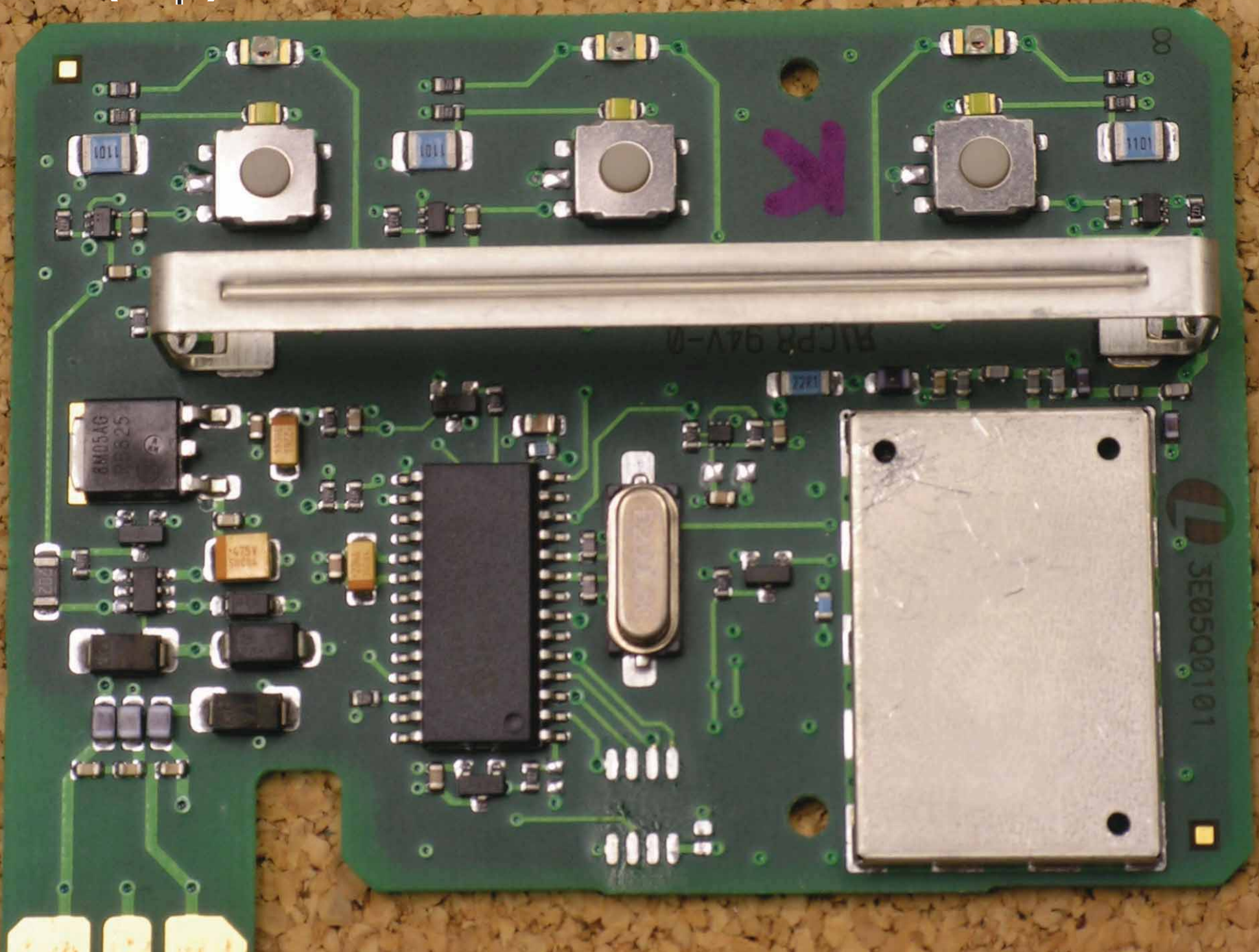
PCB (top)
