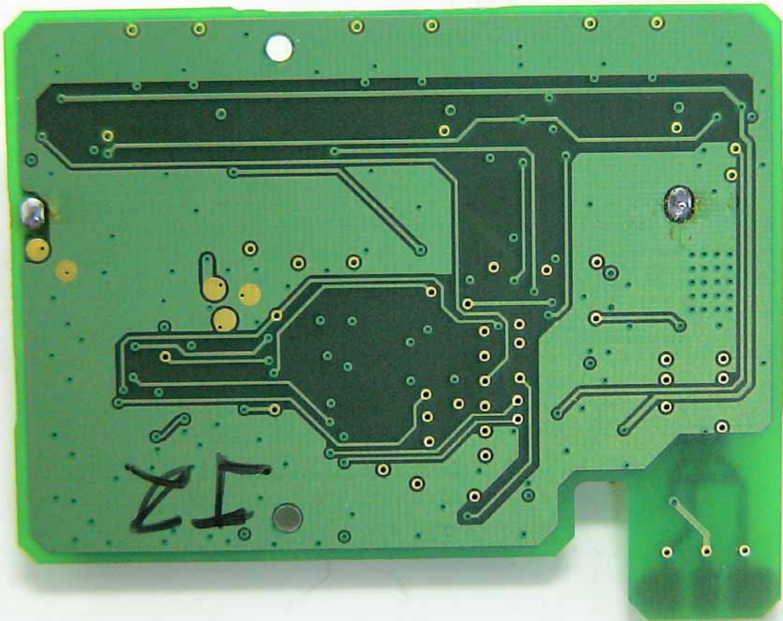
PCB (bottom)
