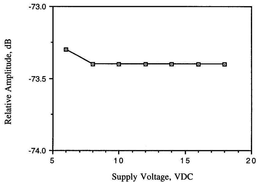
Figure 6.2. Relative emission at VCO (2xLO) vs. supply voltage.
