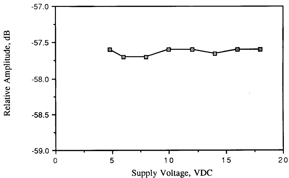
Figure 6.2. Relative emission at 651.4 MHz vs. supply voltage.
