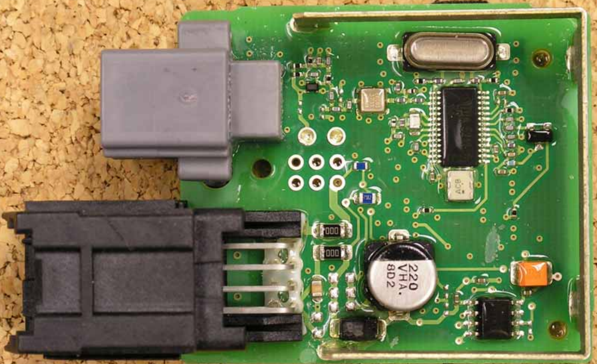
PCB (top)
