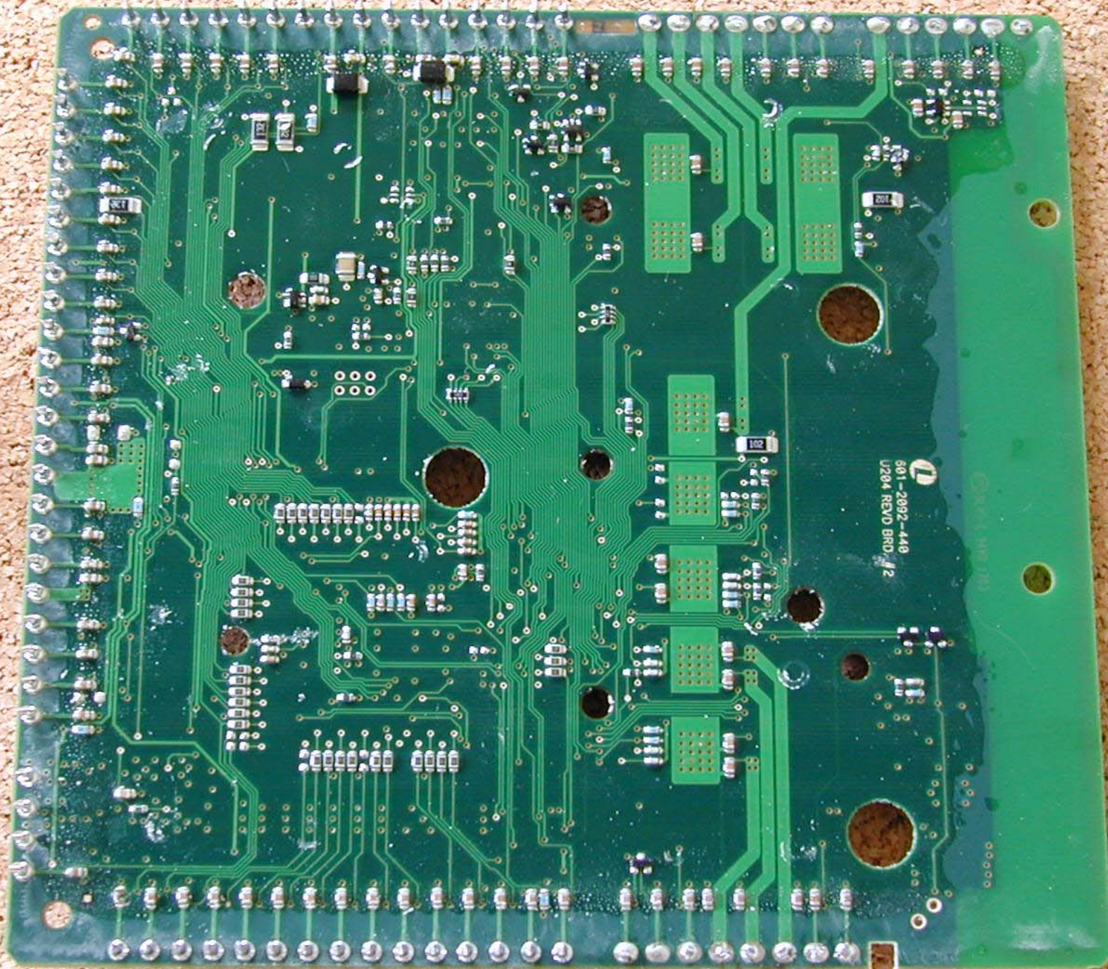
PCB 2 (bottom)
