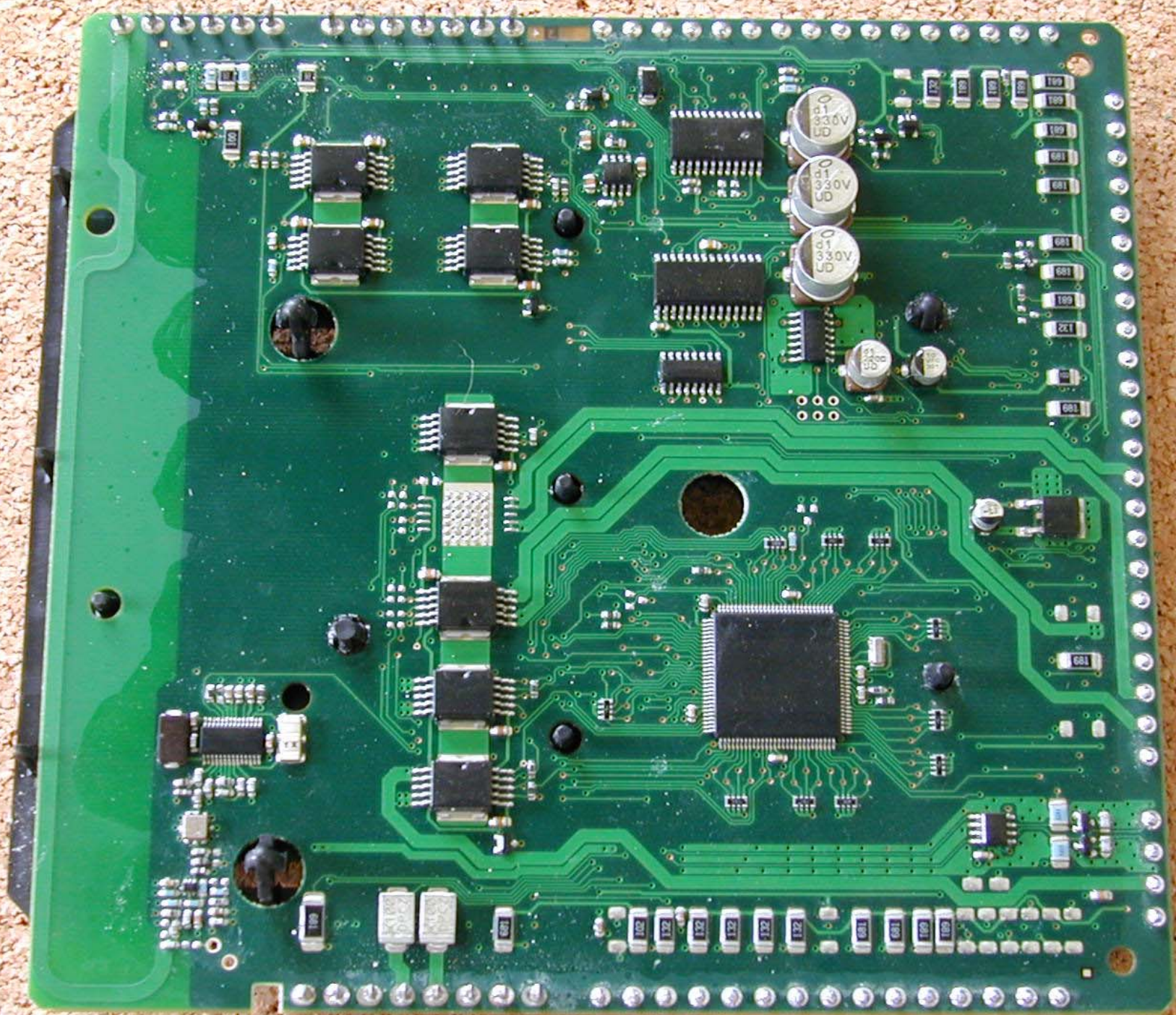
PCB 2 (top)
