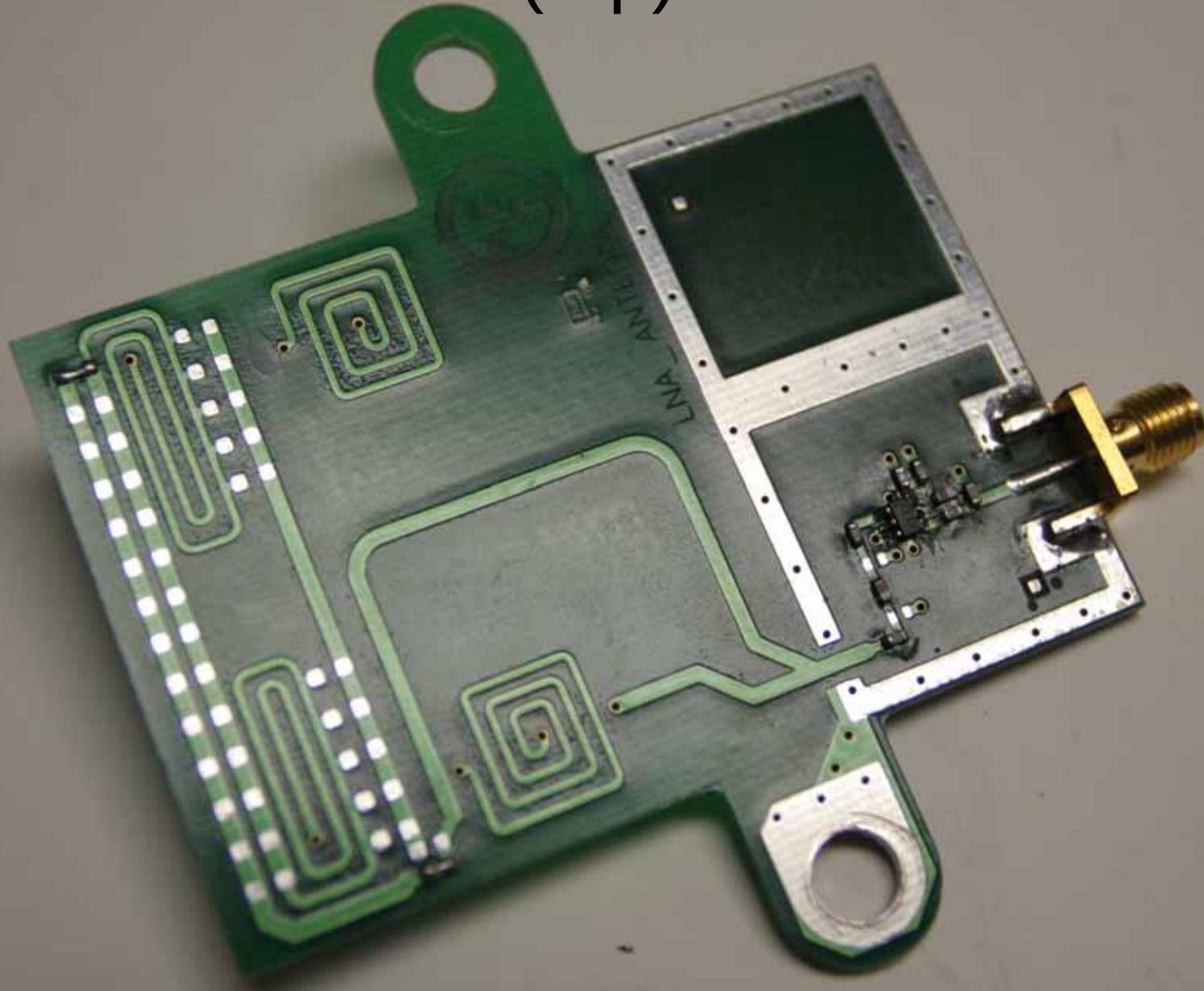
Lear Ant. PCB (top)
