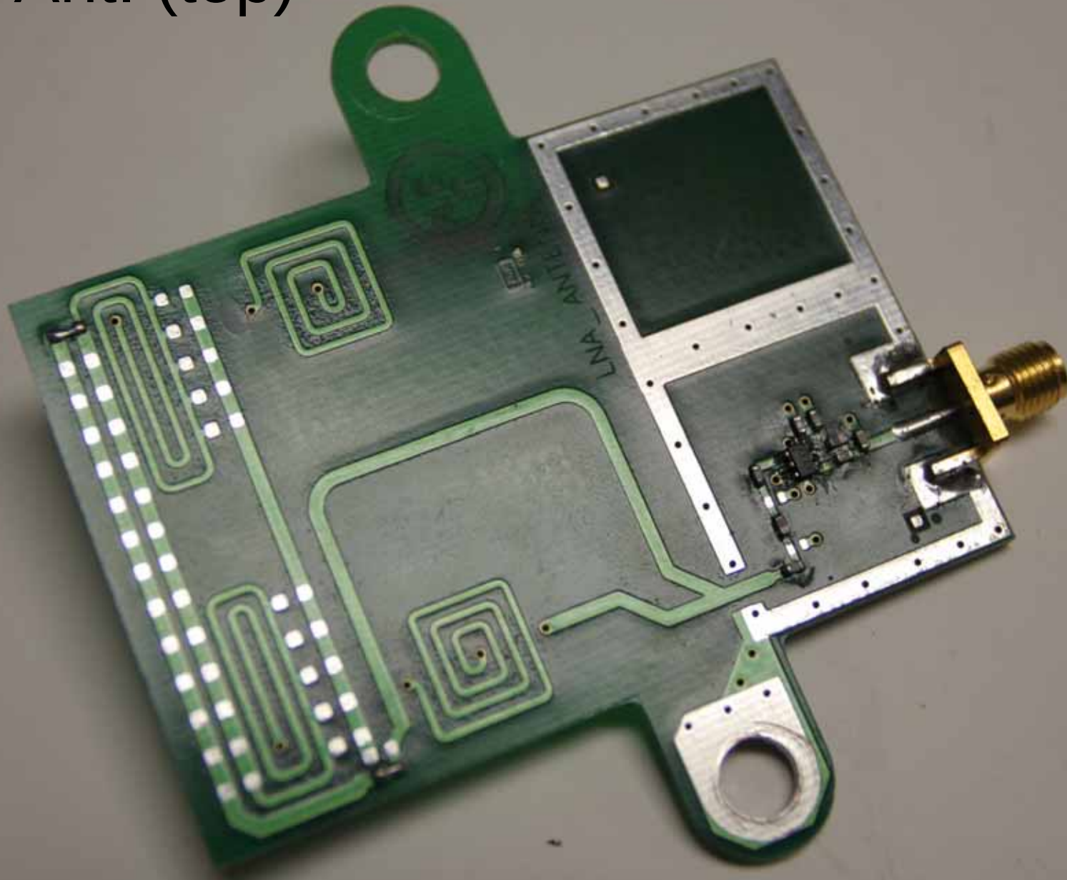
Lear Ant. (top)
