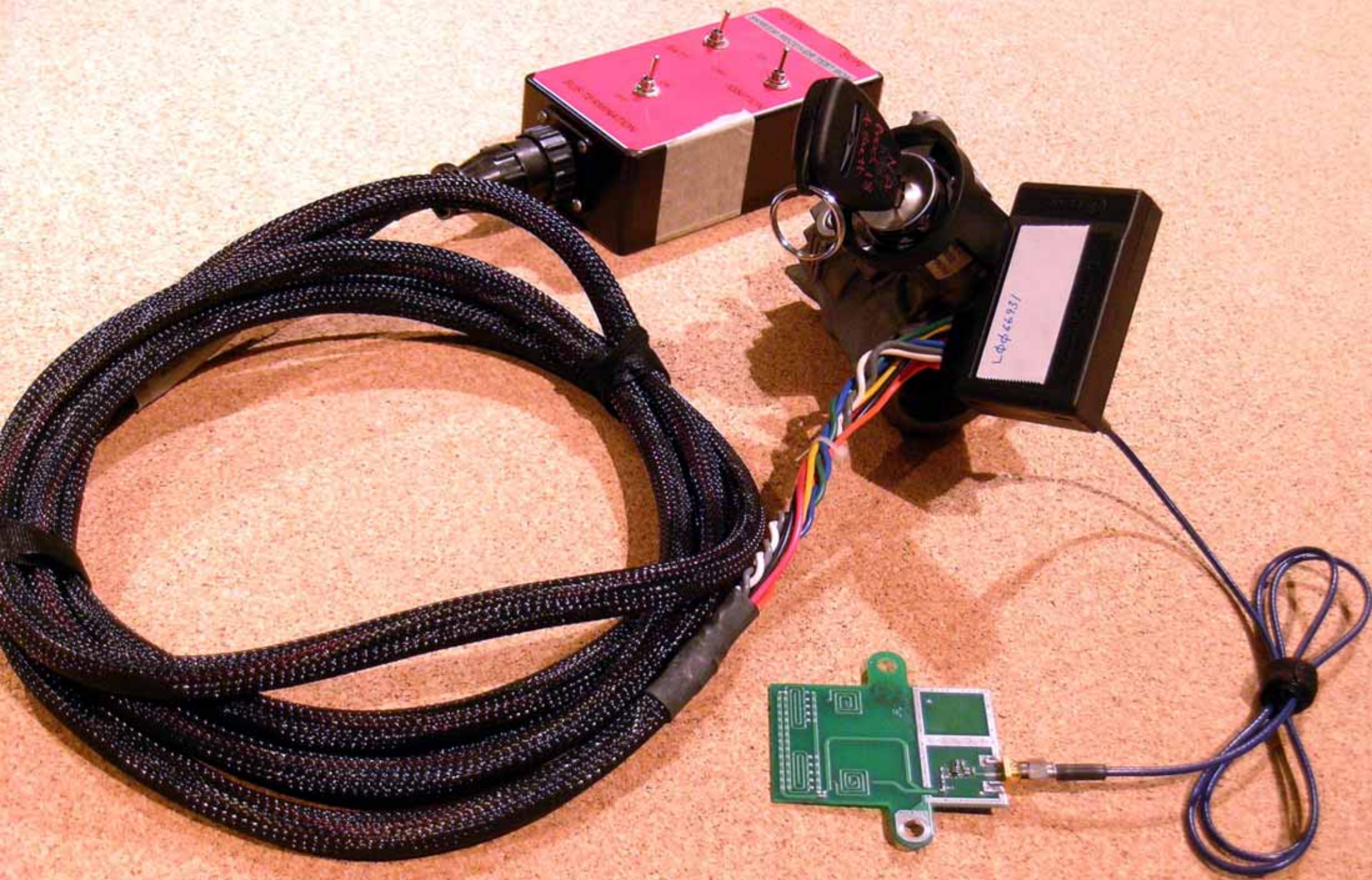
DUT with Harness (L0026931)
