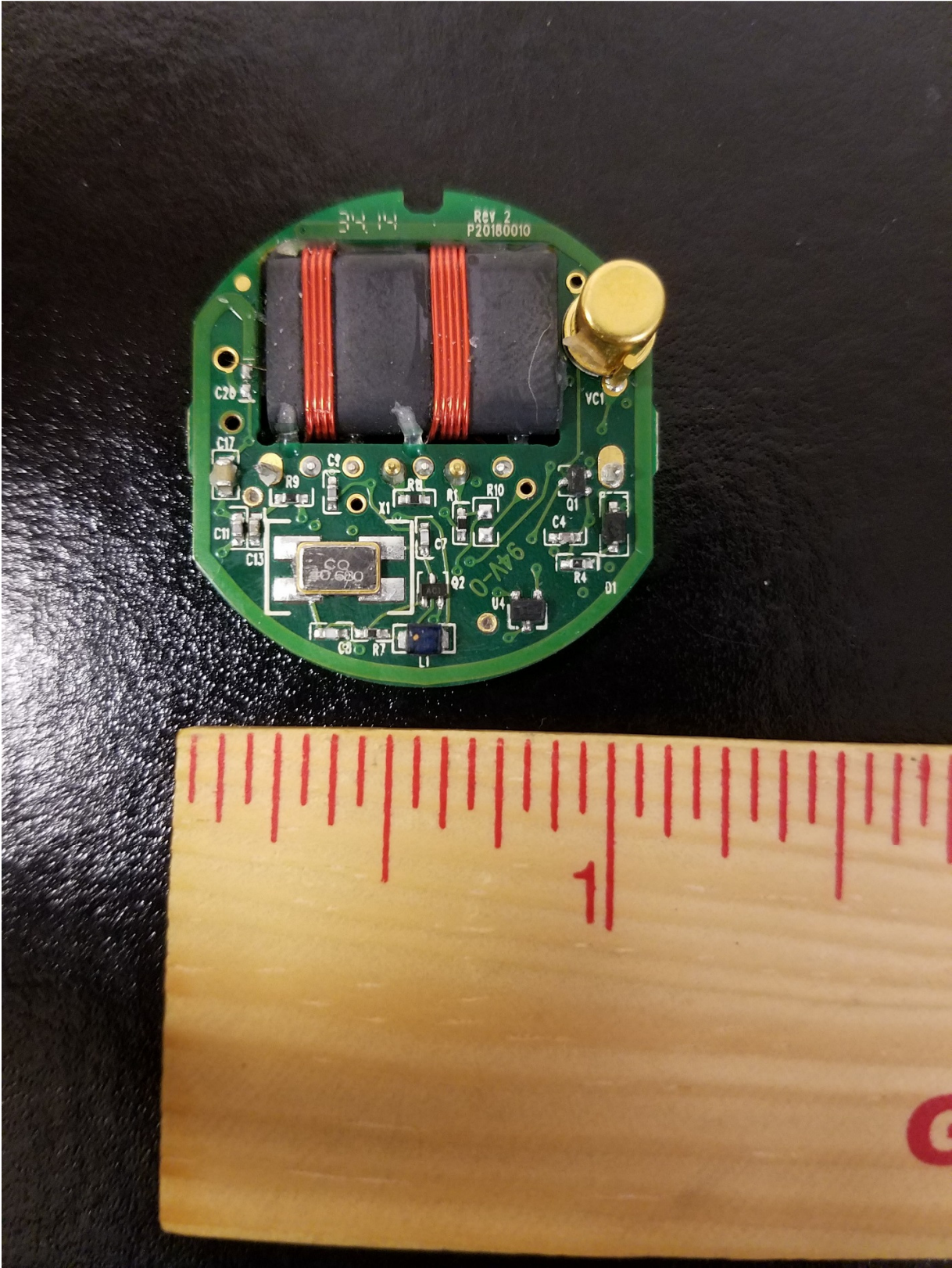
Internal bottom
