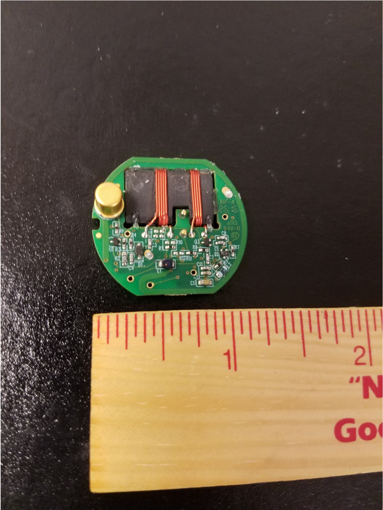
Internal bottom
