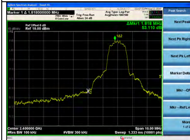
BT-8DPSK-Band Edge-Low-Non hopping
