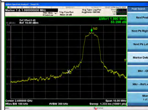
BT- \pi/4 DQPSK-Band Edge-Low-Non hopping
