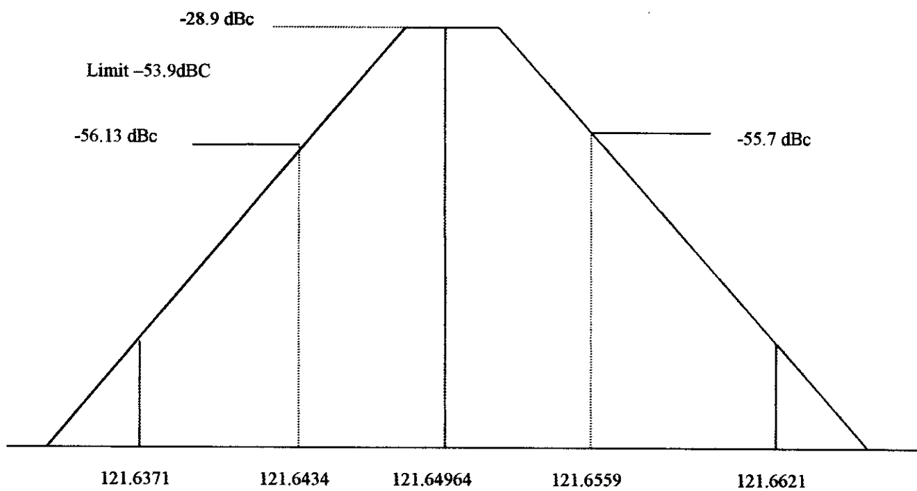
Diagram showing measured close to carrier emissions levels at 121.649 MHz
