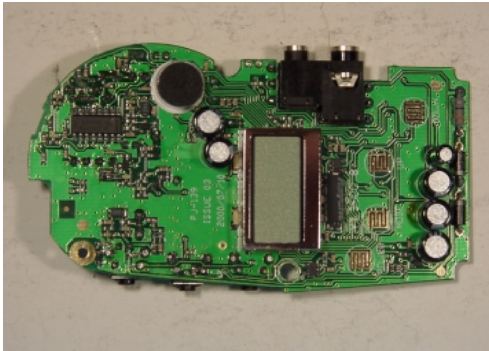
PCB Front
