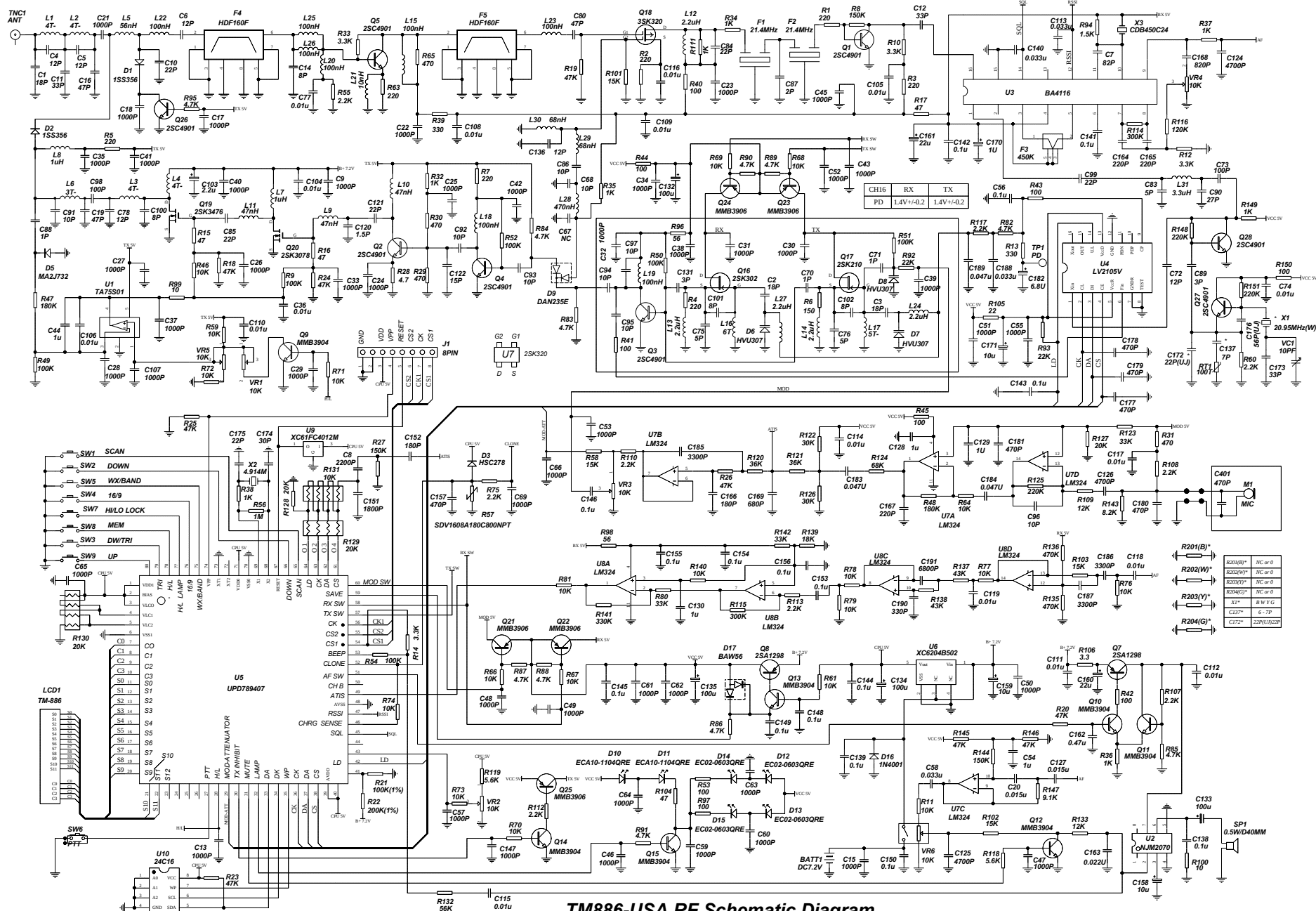
TM886-USA RF Schematic Diagram
