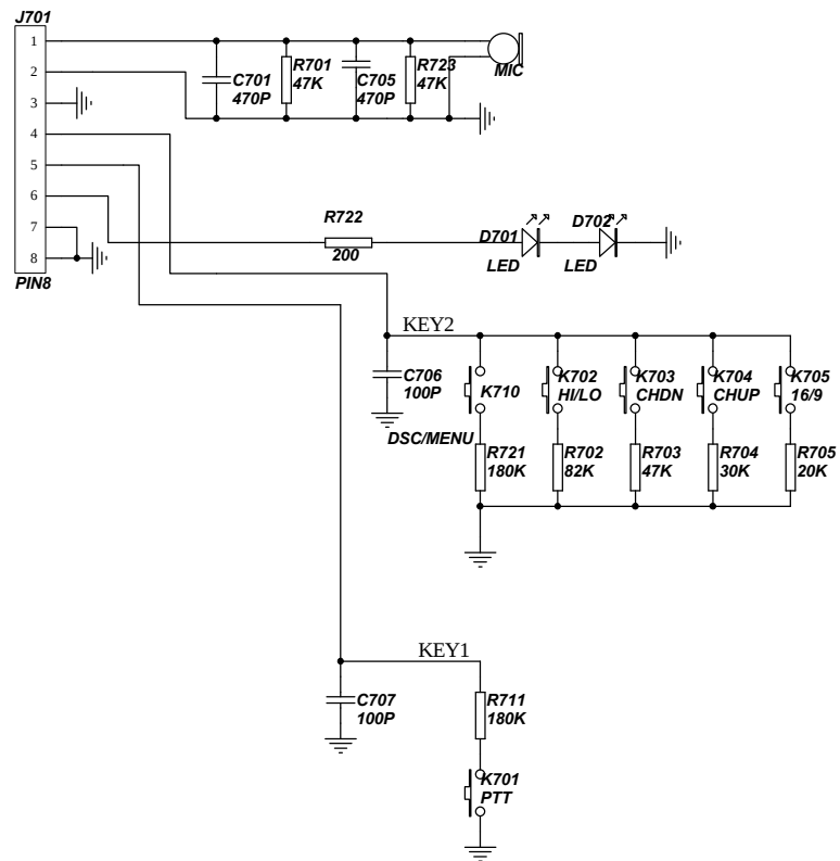
TM366-USA MIC Schematic Diagram
