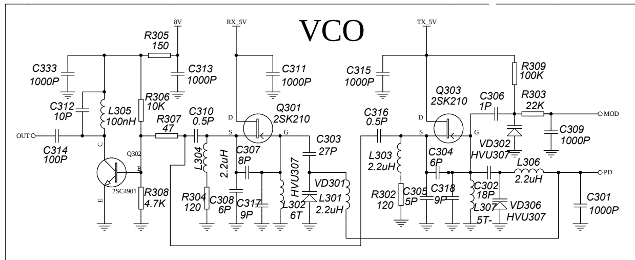
TM366-USA VCO Schematic Diagram
