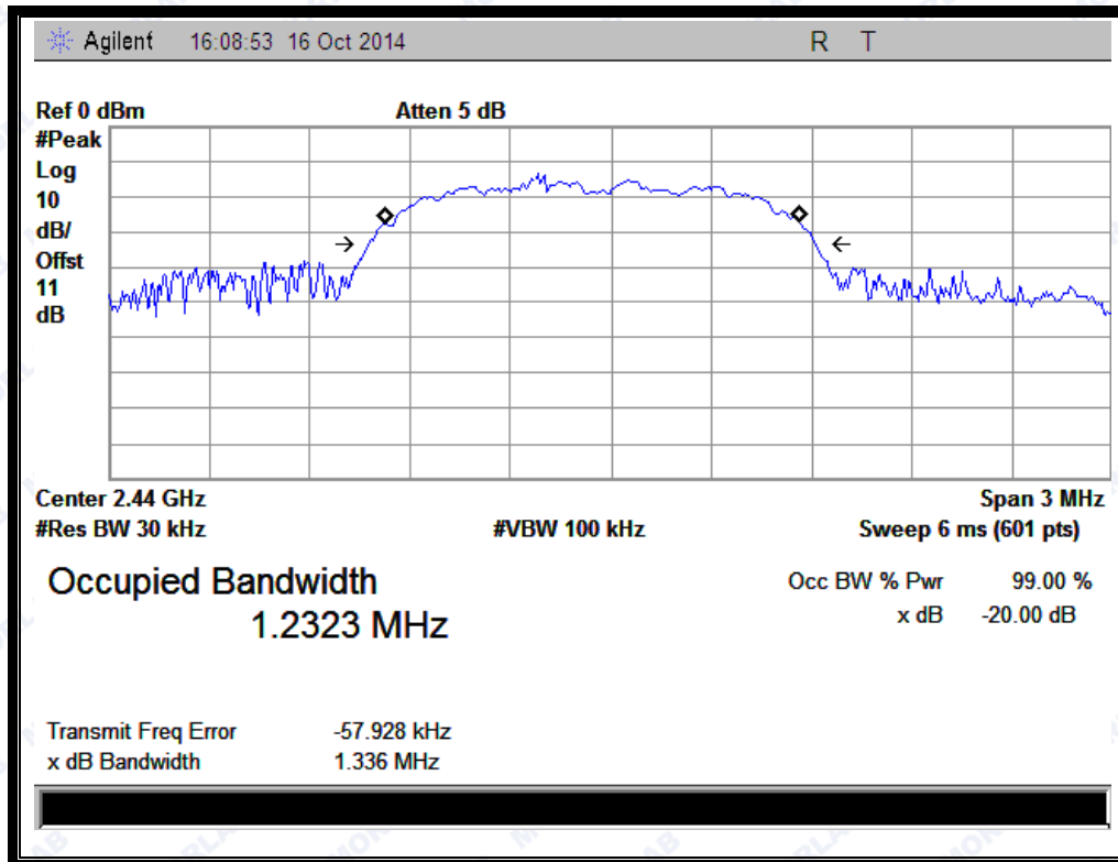
(Plot H: Channel = 2440 @ 8-DPSK)
