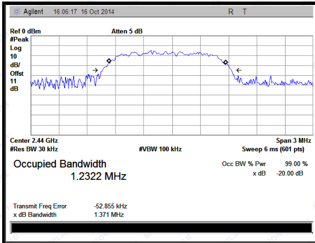
(Plot E: Channel = 2440 @ \pi/4 -DQPSK)
