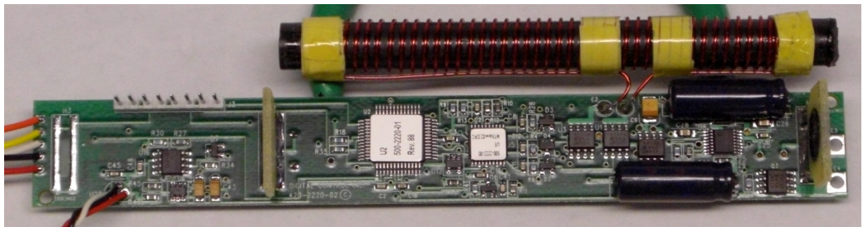
Circuit board top, antenna removed
