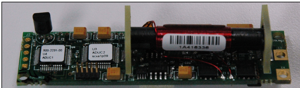
PCB Top Side 2
