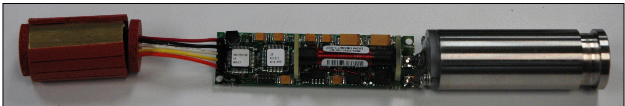
PCB with Sensor Module and Battery Housing
