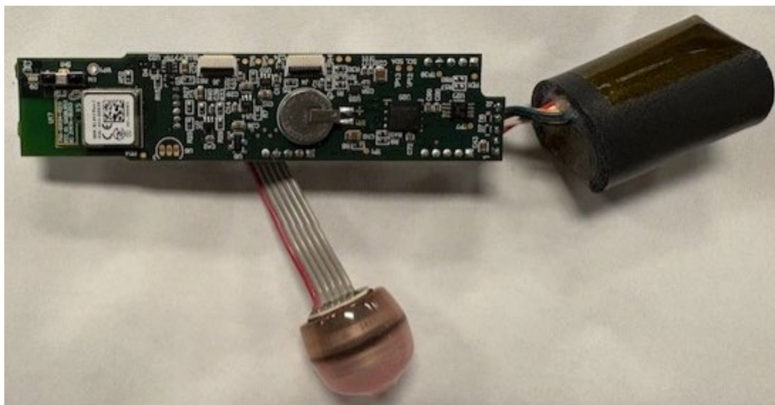
Mainboard Front
