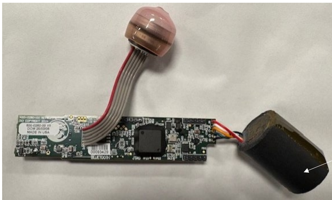
Mainboard front
