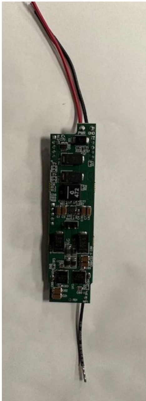
Powerboard back
