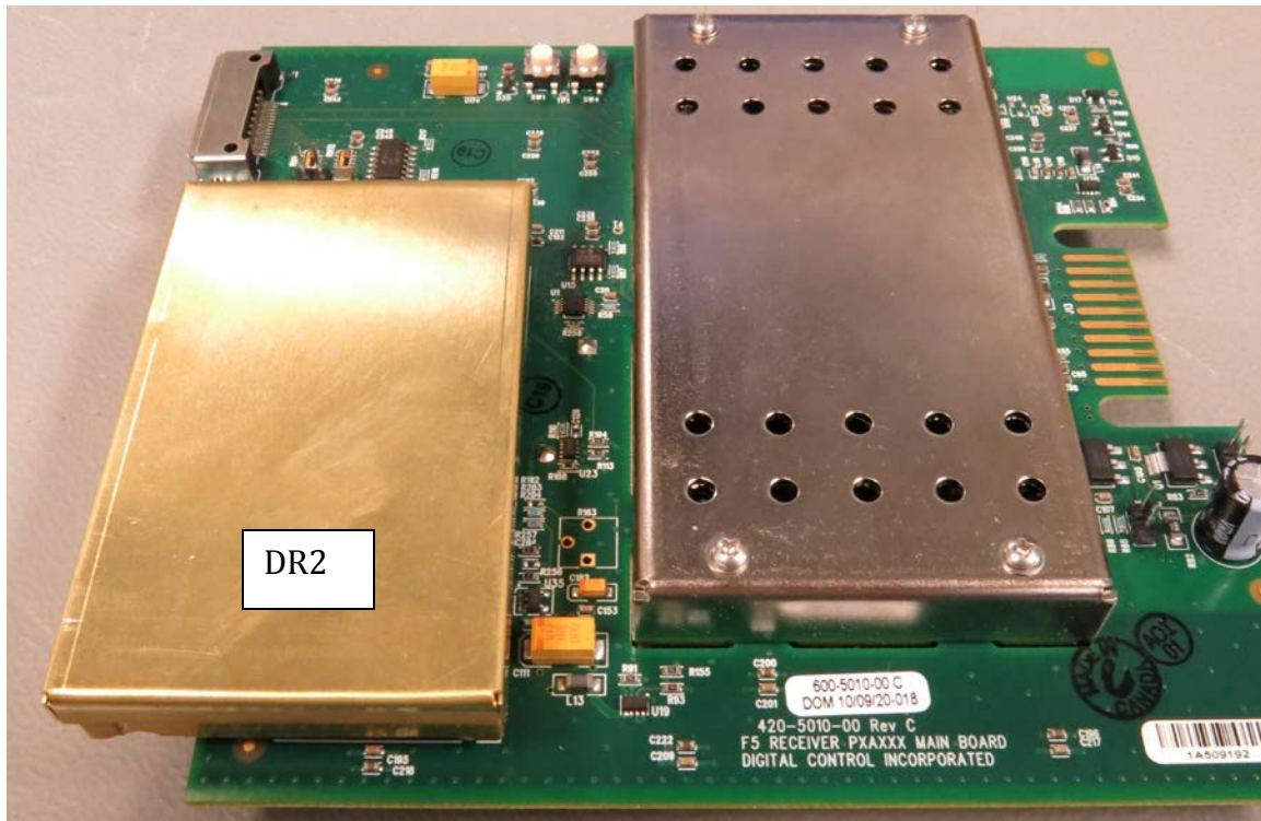
DR2 - Mounted on F5R Host Board with Shielding
