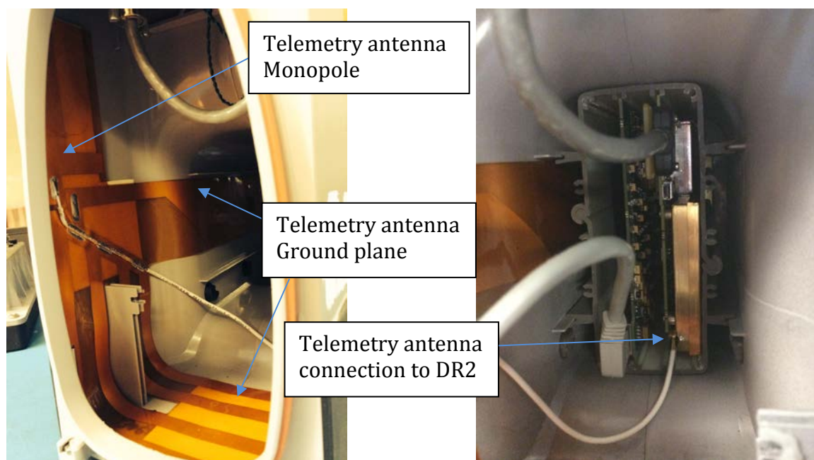
DR2 – Installed in F5R Host Device with Antenna
