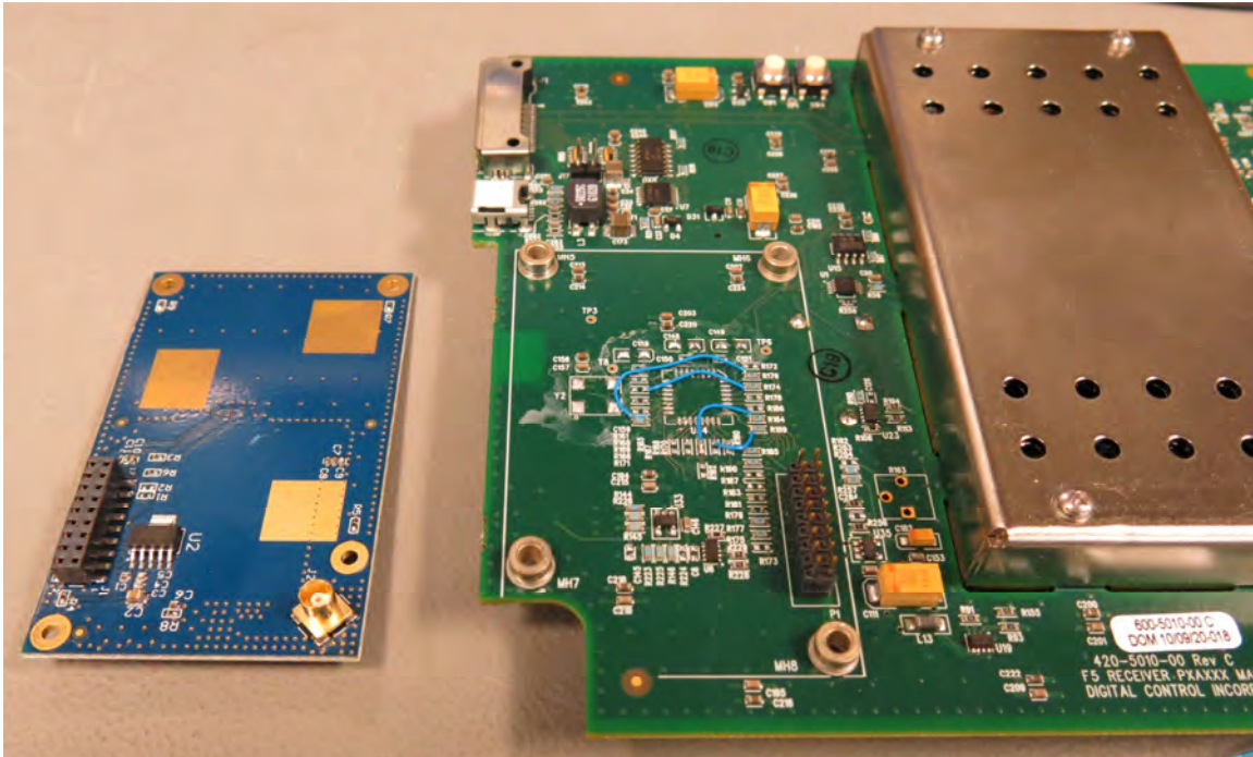
DR2 – F5R Host Board
