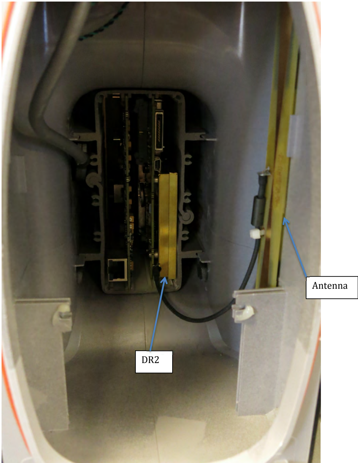
DR2 – Installed in F5R Host Device with Antenna
