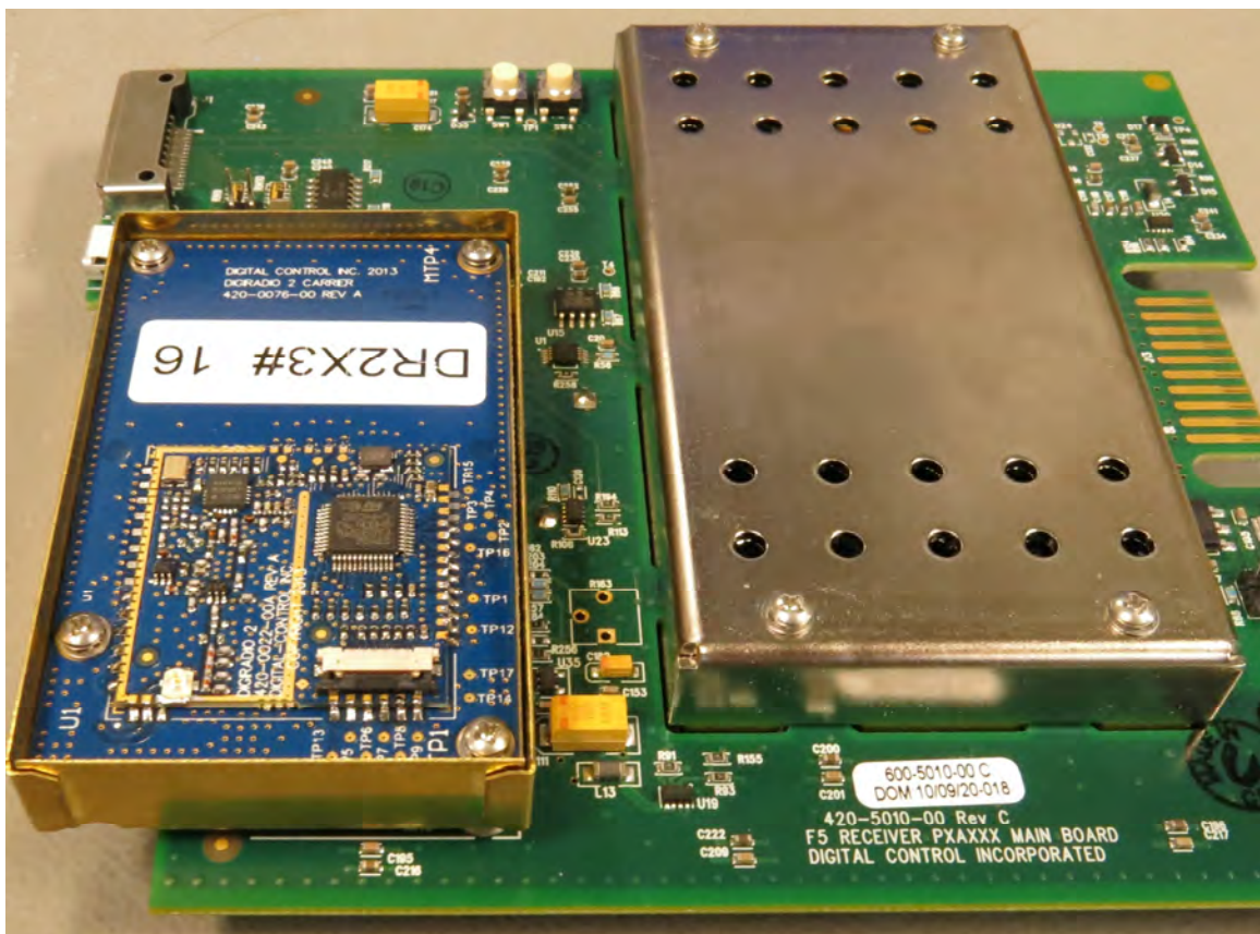
DR2 - Mounted on F5R Host Board
