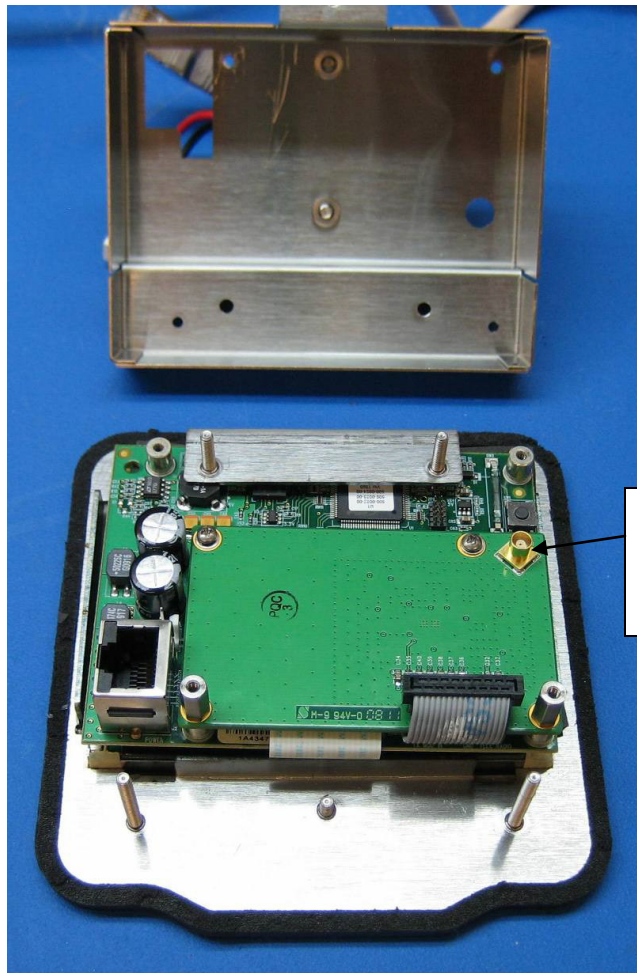
DigiRadio Module shown mounted on host pcb with display module shield can be removed
