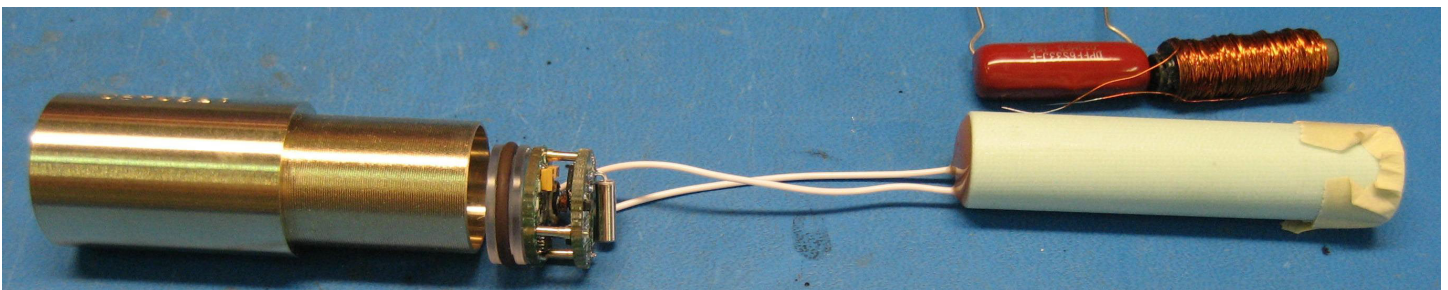
PCB assembly with antenna assembly (antenna and capacitor shown above are what is inside the small potted tube)
