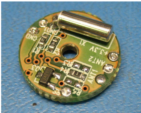
Transmitter PCB top and bottoms
