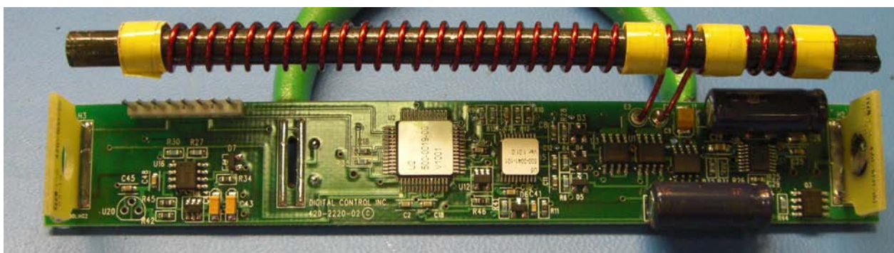
Circuit board top, antenna removed
