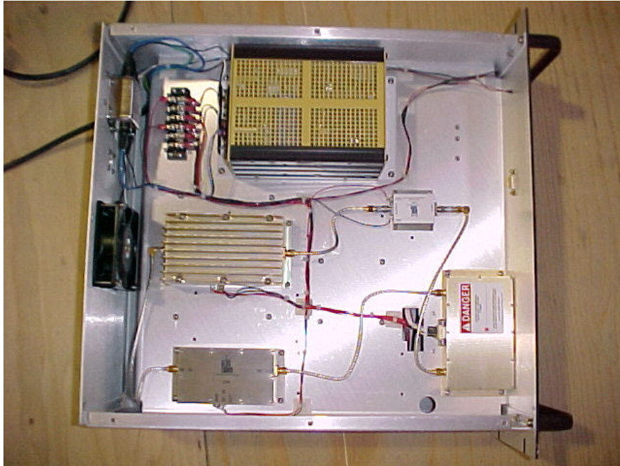
PHOTOGRAPH OF EUT – Donor Unit Bottom Inside View
