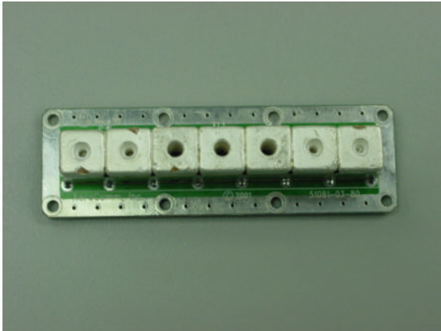
PHOTOGRAPH OF Tx Band Pass Filter Top View 882.5 MHz
