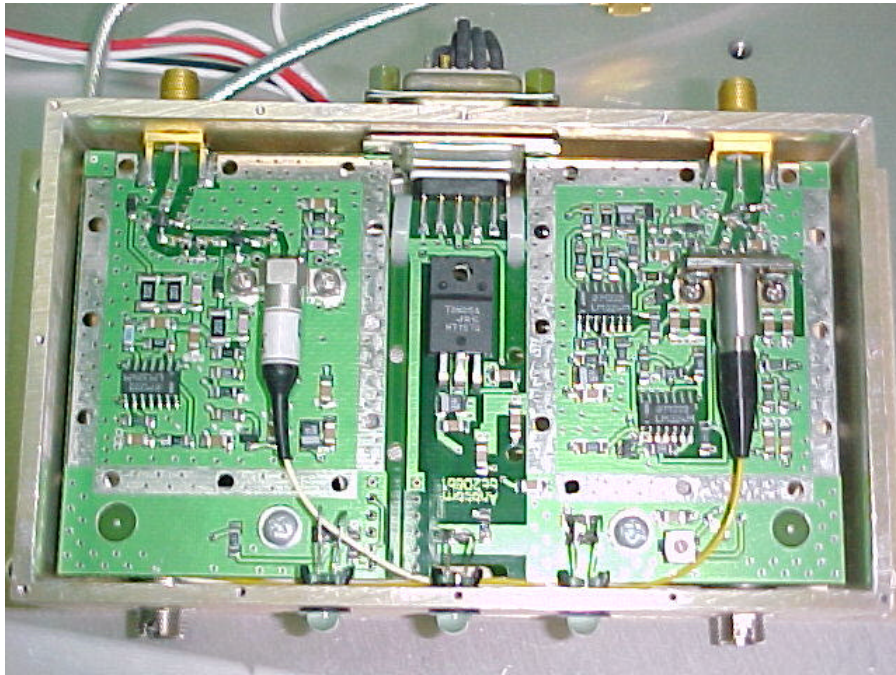
PHOTOGRAPH OF Class 3b Laser Product Soldering Side Model: AC231-A1, S/N 7760122017
