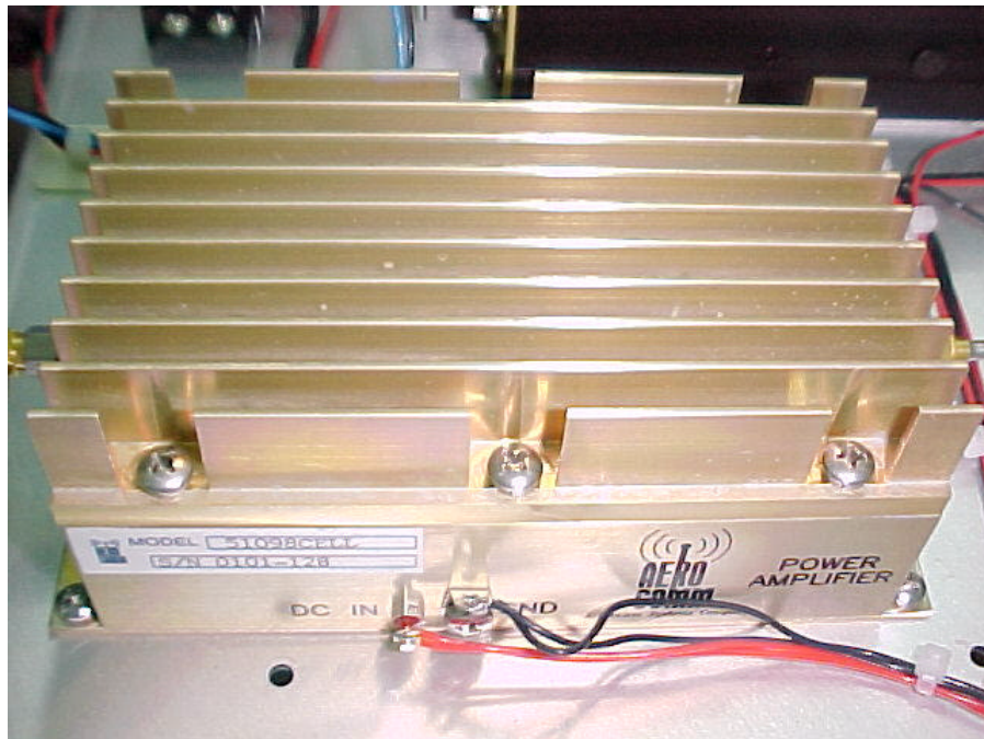
PHOTOGRAPH OF Power Amplifier Component Side View Model: 51098CELL, S/N 0101-128
