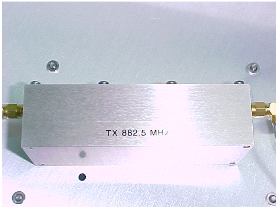
PHOTOGRAPH OF Tx Band Pass Filter Whole View 882.5 MHz
