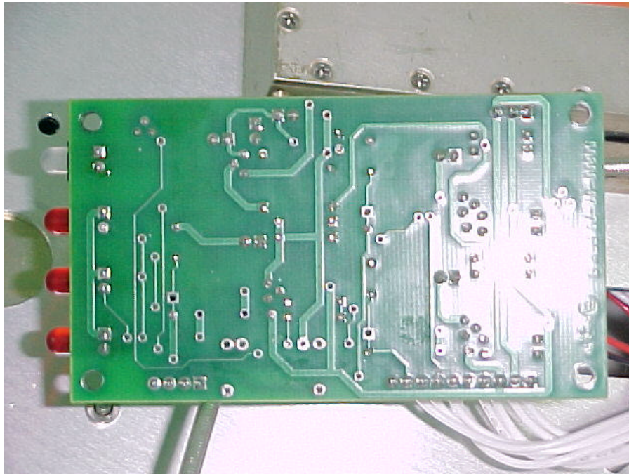
PHOTOGRAPH OF Alarm Indicator Board Soldering Side S/N 50800-03-70
