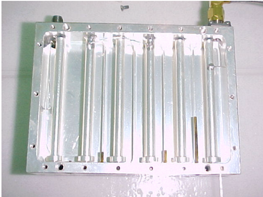
PHOTOGRAPH OF Fiber Product and Sub System Inside View Model: DC0040, S/N 0983
