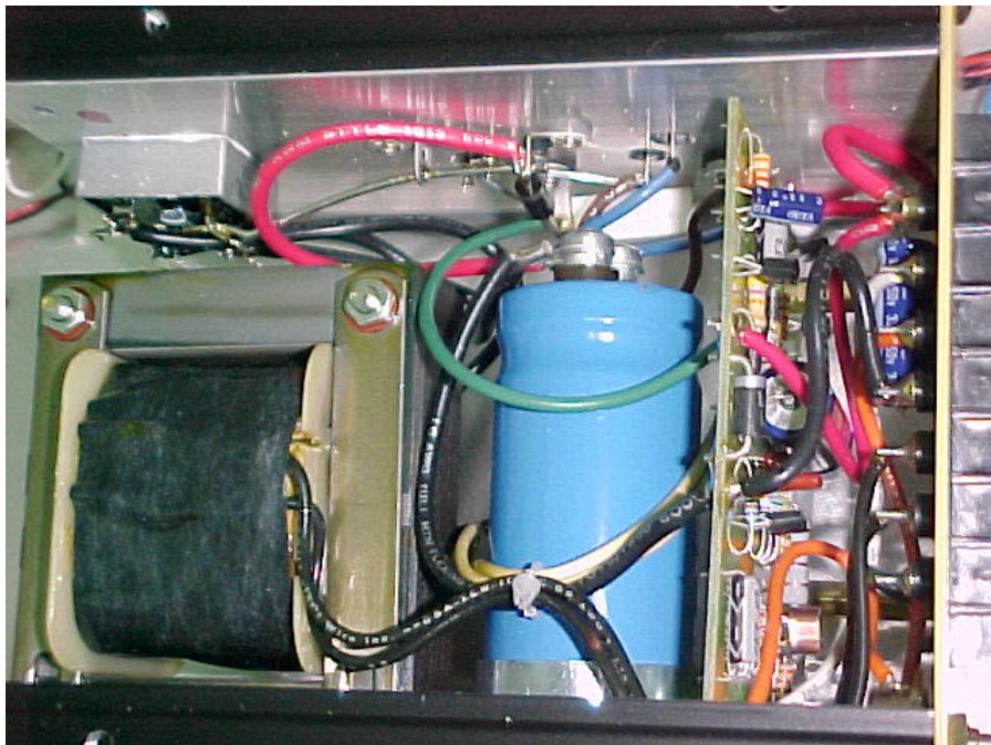
PHOTOGRAPH OF Power Supply Component Side Model: A12MT400M
