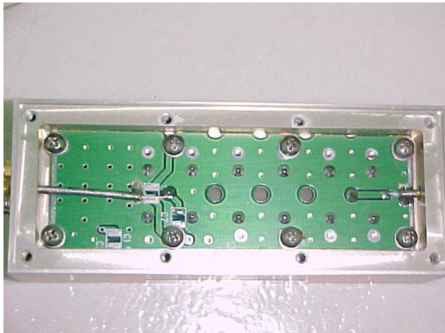
PHOTOGRAPH OF Tx Band Pass Filter Bottom View 882.5 MHz
