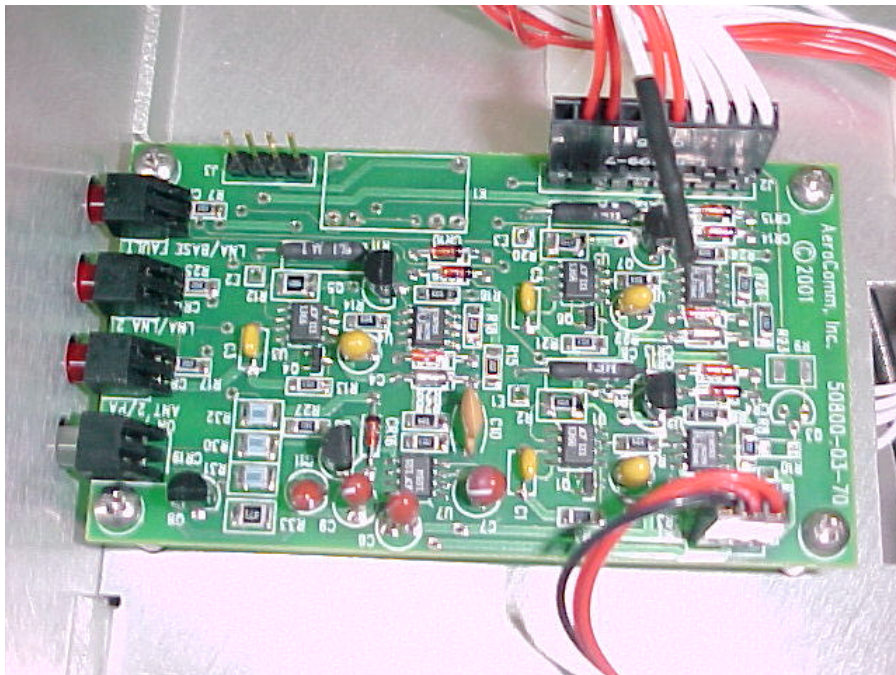
PHOTOGRAPH OF Alarm Indicator Board Component Side S/N 50800-03-70
