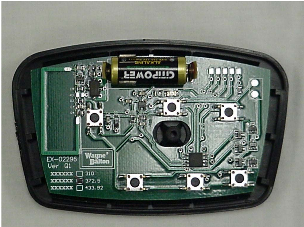
Photo 3. Internal View, Top Side
