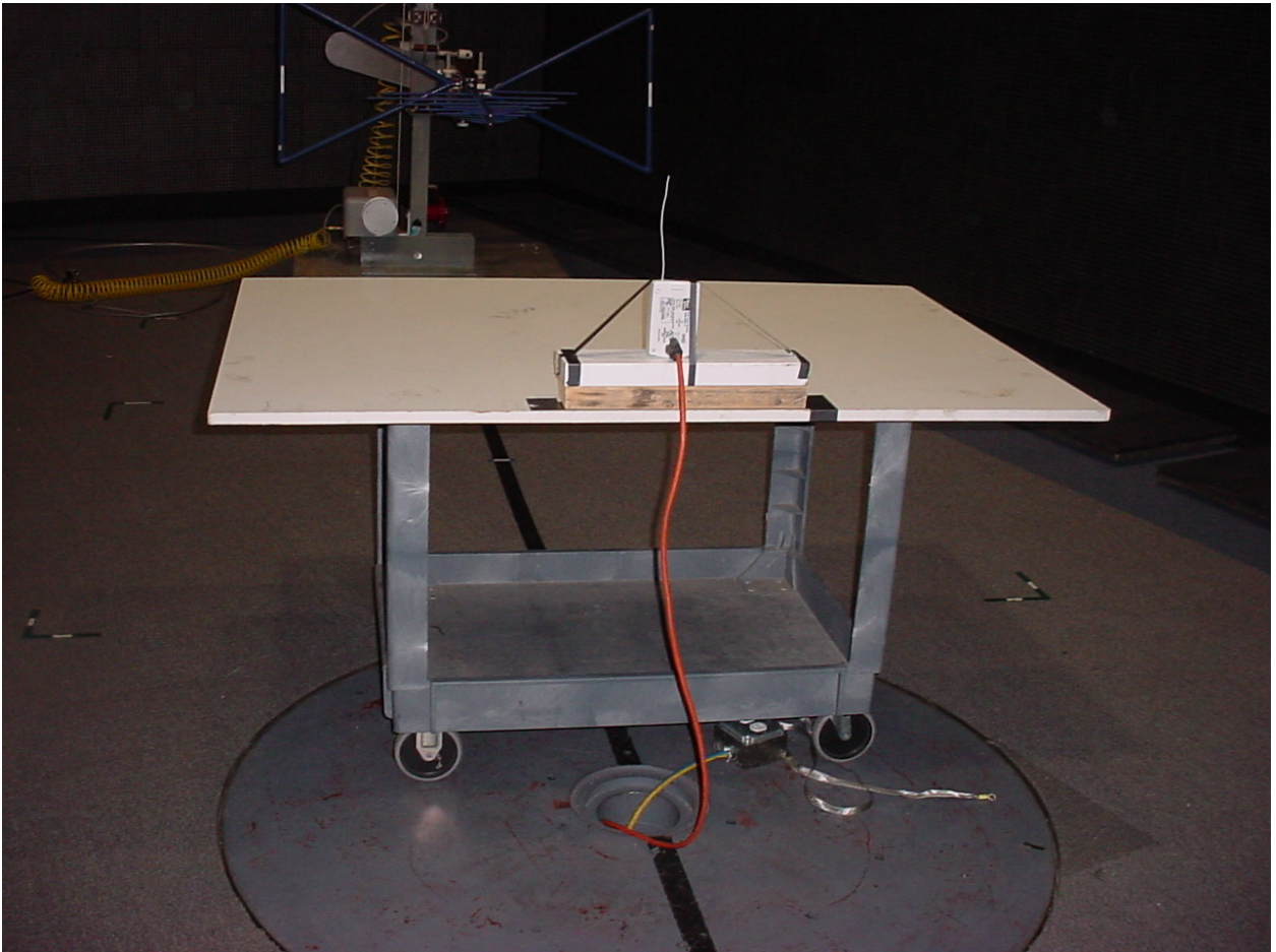
Figure 5: Test Setup – Radiated Emissions - Unintentional
