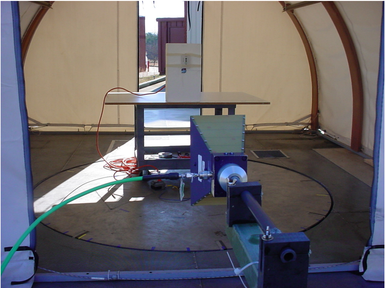
Figure 3: Test Setup – Radiated Emissions
