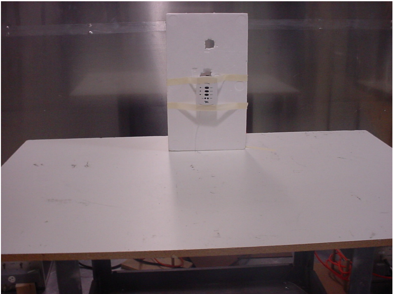
Figure 6: Test Setup – Conducted Emissions
