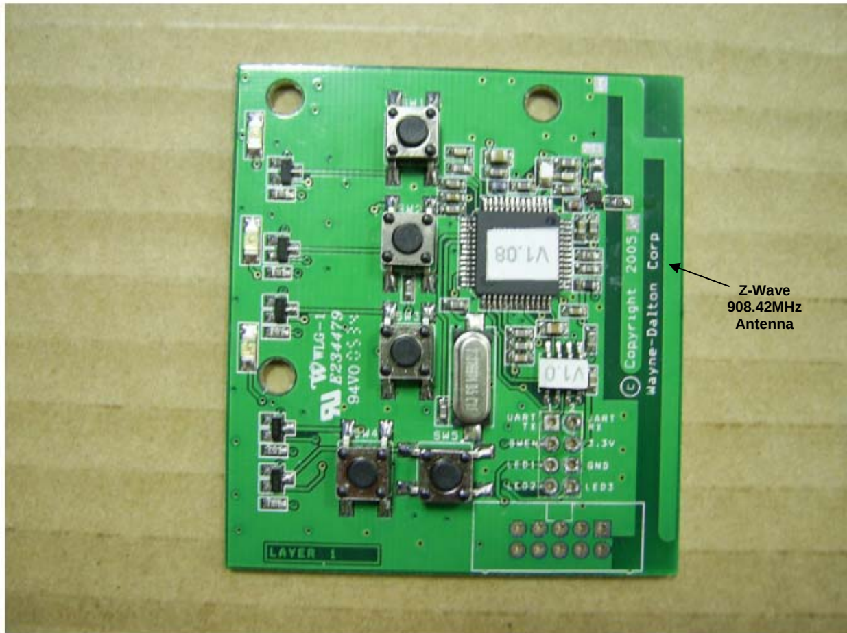
Figure 1: Internal – Front View – Z-Wave Board
