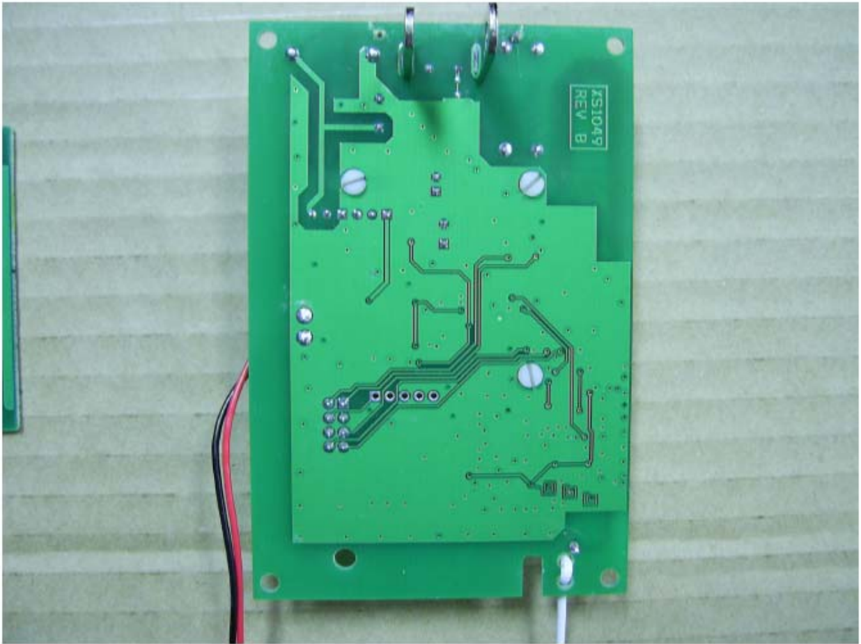
Figure 4: Internal – Back View - PIC PCB (372MHz)
