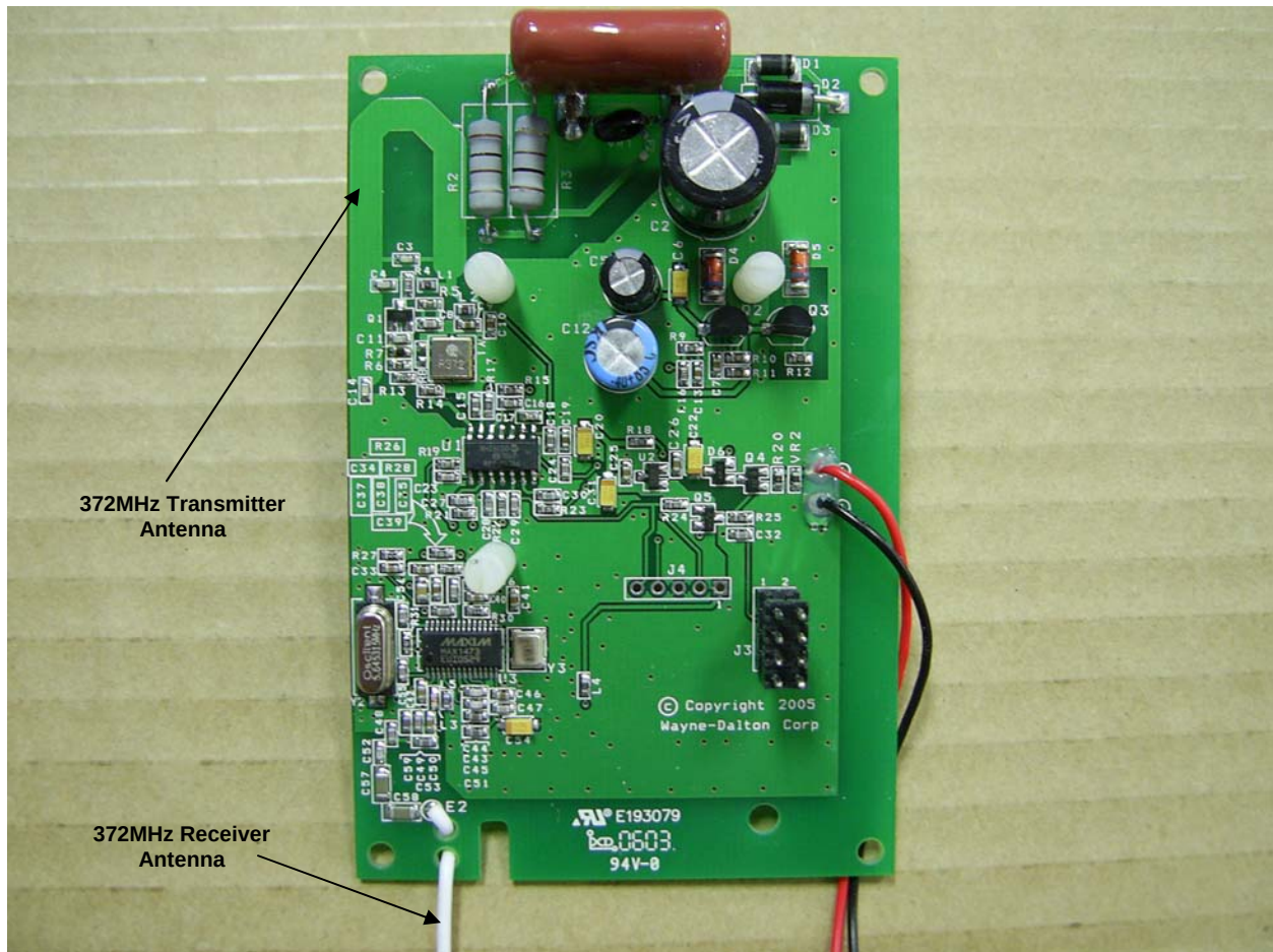
Figure 3: Internal – Front View – PIC PCB (372MHz)
