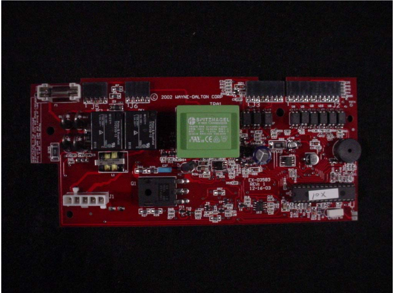
Figure 2: Motor Control/433.92MHz Transmitter Board – Top View
