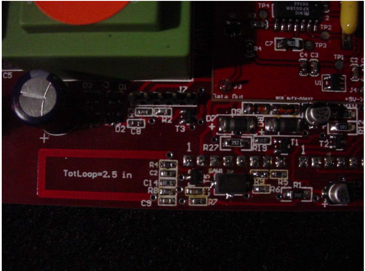
Figure 7: Transmitter Circuitry
