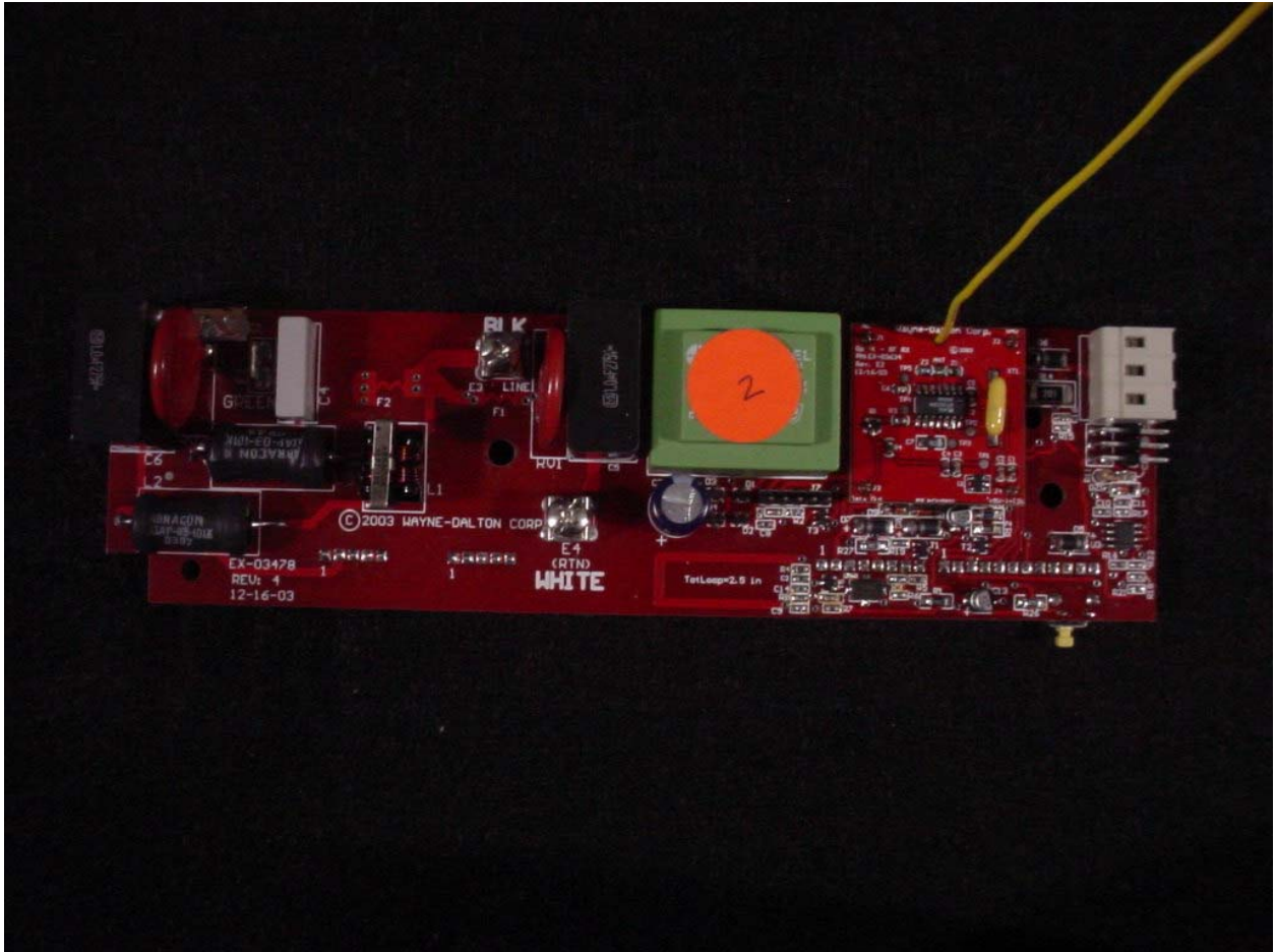
Figure 4: Receiver Board – Top View
