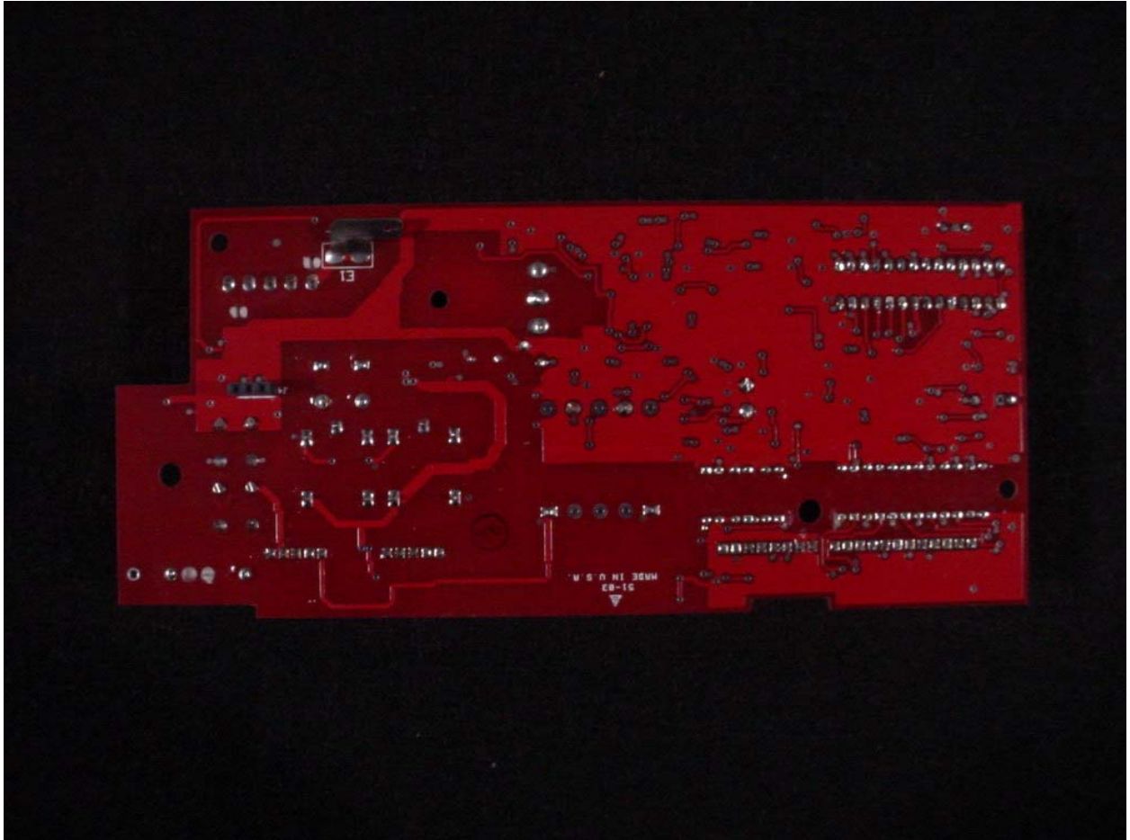
Figure 3: Motor Control/433.92MHz Transmitter Board – Bottom View
