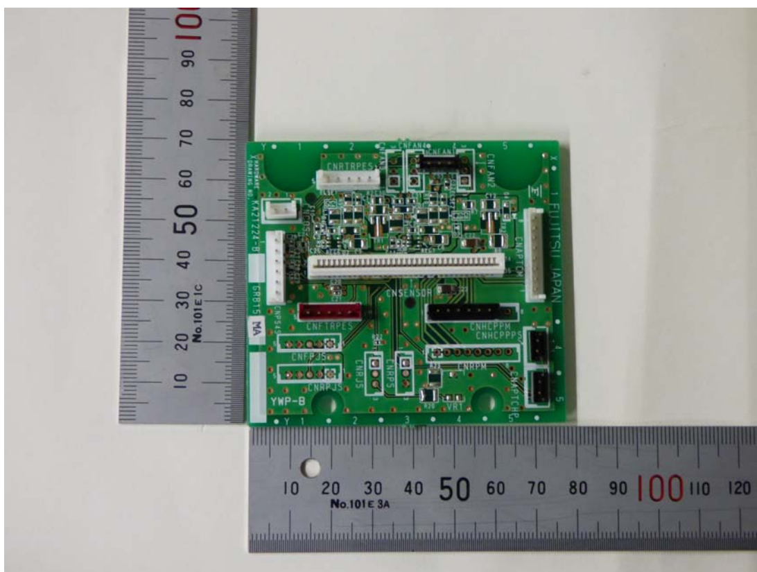
[Relay board, top side]
