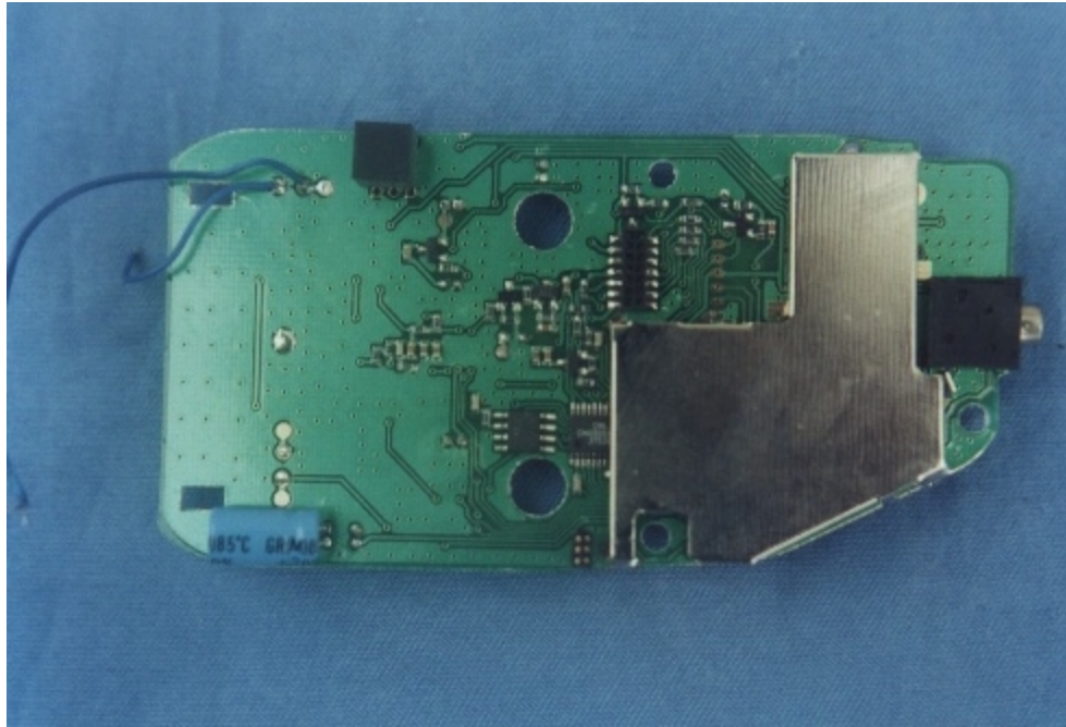
Figure 7. General Appearance of the PCB
