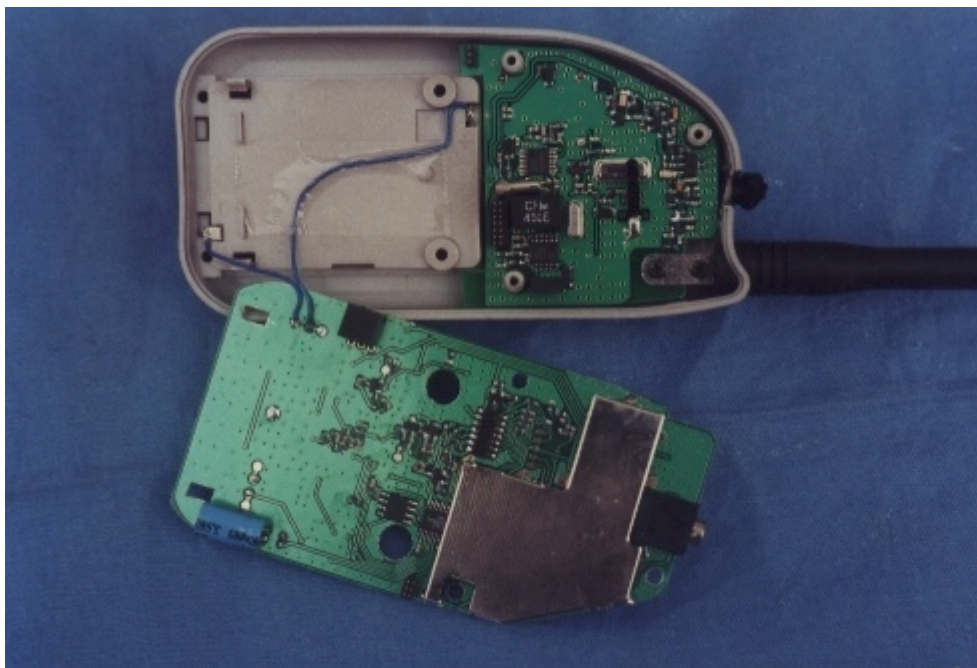
Figure 4. Cover Opened
