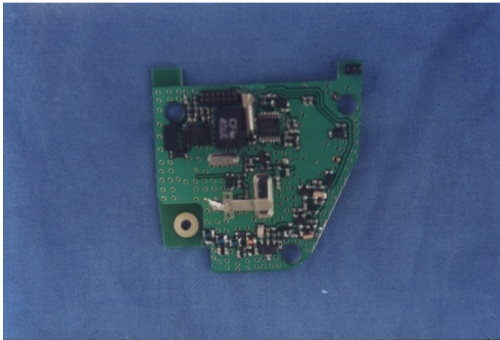
Figure 8. General Appearance of the PCB
