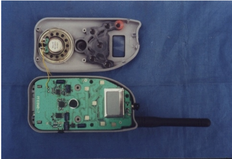
Figure 3. Cover Opened
