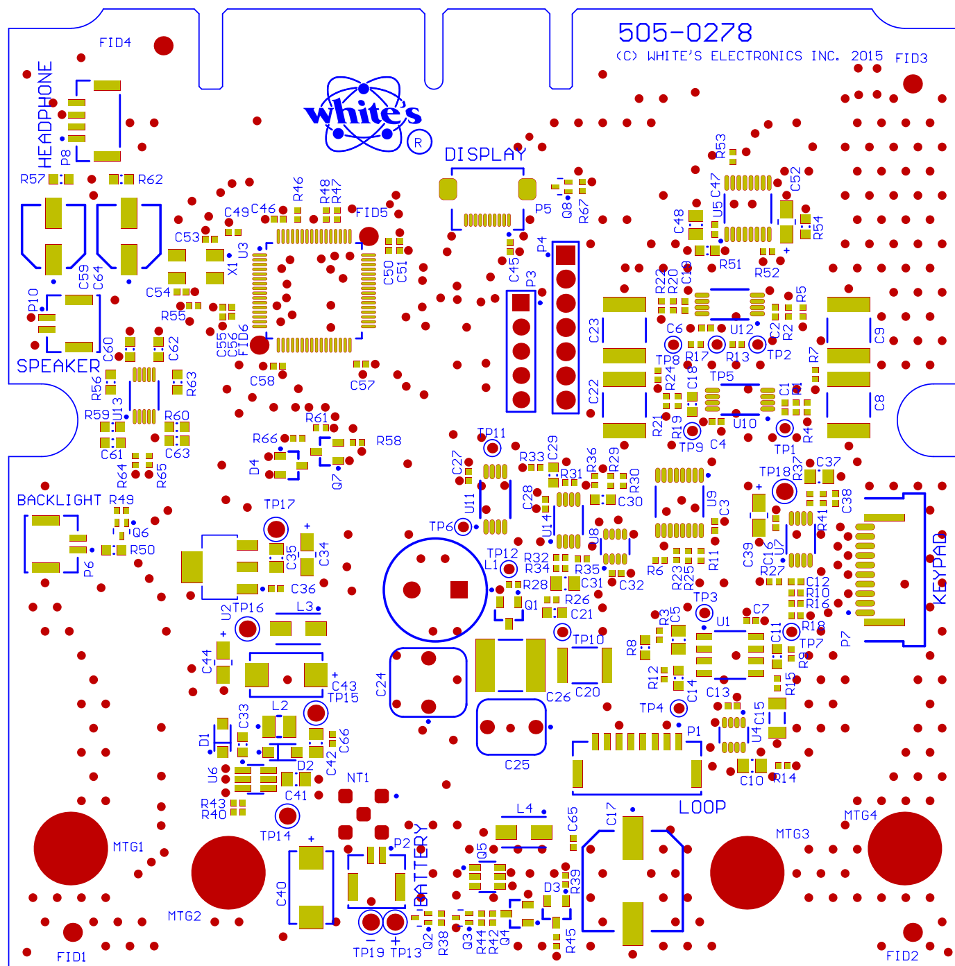
TOP OVERLAY SILK SCREEN FOR 505-0278 AS VIEWED FROM THE TOP LAYER
