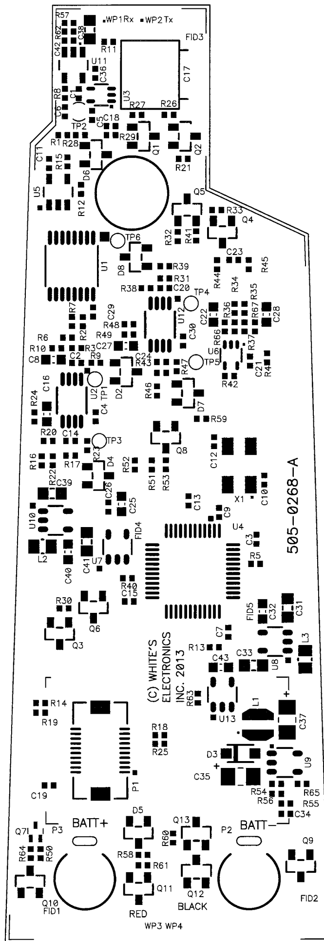
TOP SOLDER MASK FOR 505-0268-A AS VIEWED FROM THE COM
