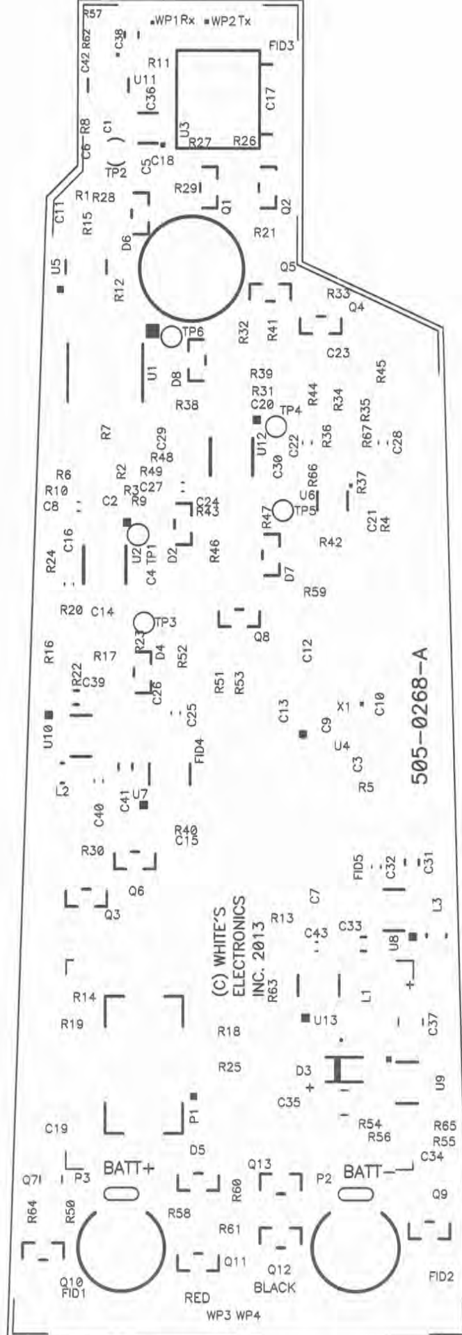
SILK SCREEN FOR 505-0268-A AS VIEWED FROM THE COMPONE
