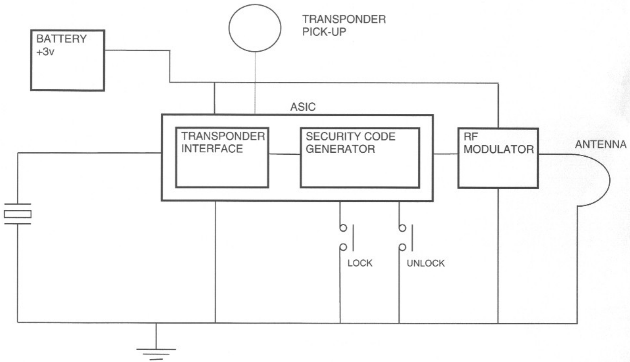
17TN Block Diagram
